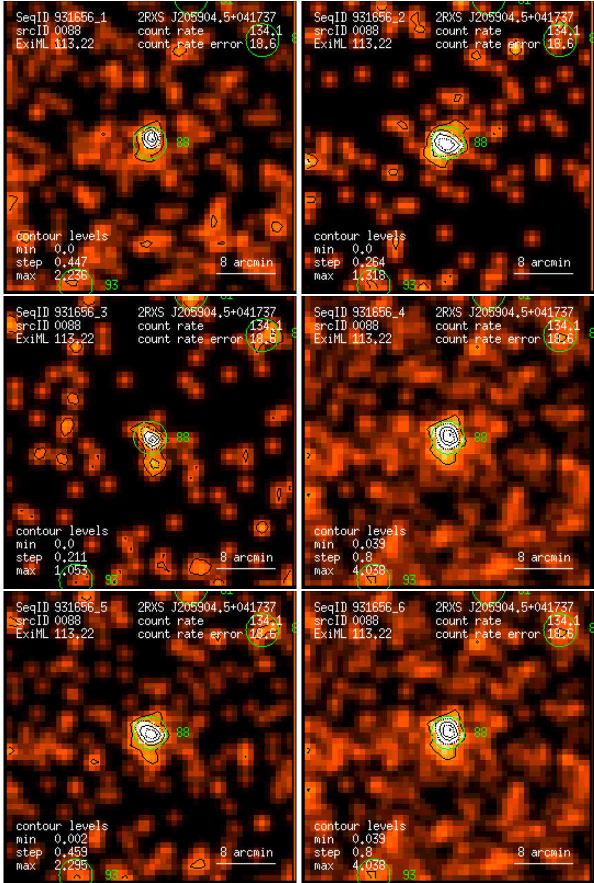
Figure 88: RASS 931656: detection 0088: band rate images, Gaussian filter: (1) PSPC channels 11 – 41, (2) 52 – 90, (3) 91 – 201, (4) 11 – 235, (5) 52 – 201, (6) 11 – 201. Broad band rates in counts/ks. Band rate contour levels in counts/ks/arcmin 2 .
