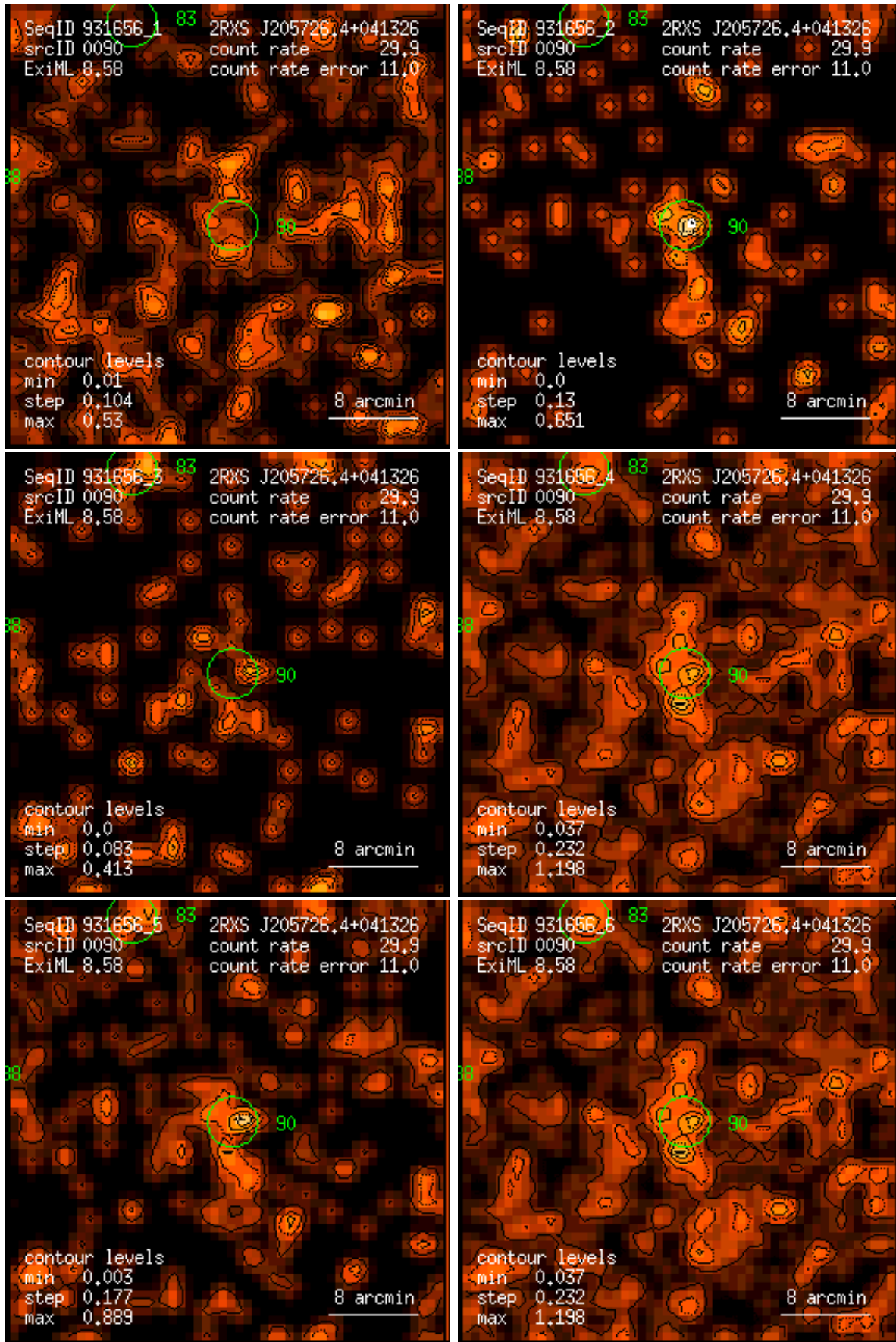
Figure 90: RASS 931656: detection 0090: band rate images, Gaussian filter: (1) PSPC channels 11 – 41, (2) 52 – 90, (3) 91 – 201, (4) 11 – 235, (5) 52 – 201, (6) 11 – 201. Broad band rates in counts/ks. Band rate contour levels in counts/ks/arcmin 2 .
