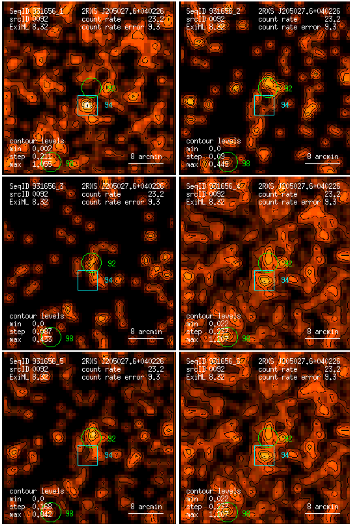
Figure 92: RASS 931656: detection 0092: band rate images, Gaussian filter: (1) PSPC channels 11 – 41, (2) 52 – 90, (3) 91 – 201, (4) 11 – 235, (5) 52 – 201, (6) 11 – 201. Broad band rates in counts/ks. Band rate contour levels in counts/ks/arcmin 2 .
