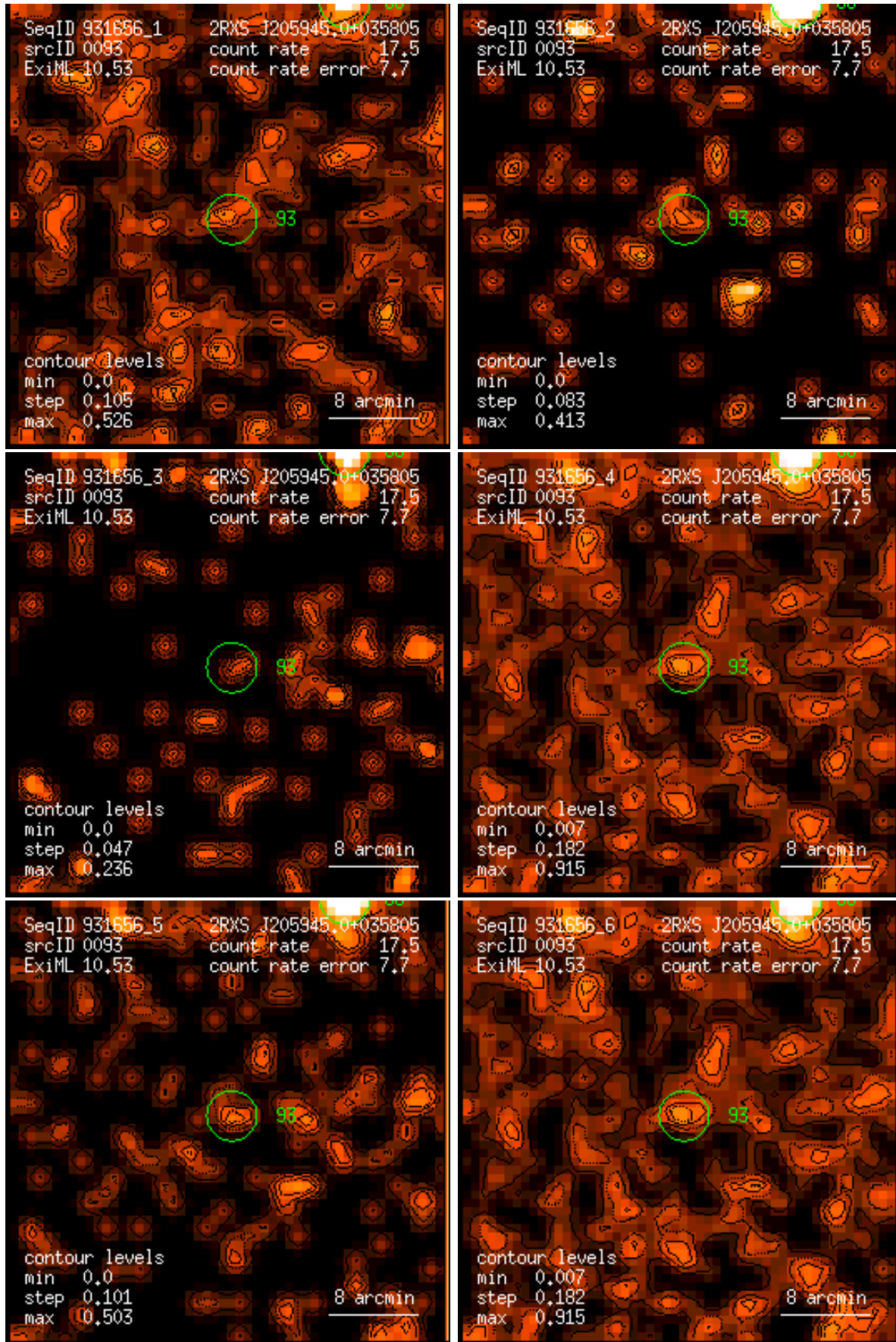
Figure 93: RASS 931656: detection 0093: band rate images, Gaussian filter: (1) PSPC channels 11 – 41, (2) 52 – 90, (3) 91 – 201, (4) 11 – 235, (5) 52 – 201, (6) 11 – 201. Broad band rates in counts/ks. Band rate contour levels in counts/ks/arcmin 2 .
