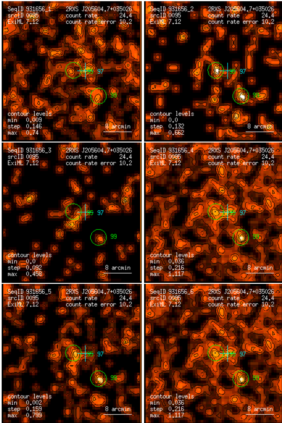
Figure 95: RASS 931656: detection 0095: band rate images, Gaussian filter: (1) PSPC channels 11 – 41, (2) 52 – 90, (3) 91 – 201, (4) 11 – 235, (5) 52 – 201, (6) 11 – 201. Broad band rates in counts/ks. Band rate contour levels in counts/ks/arcmin 2 .
