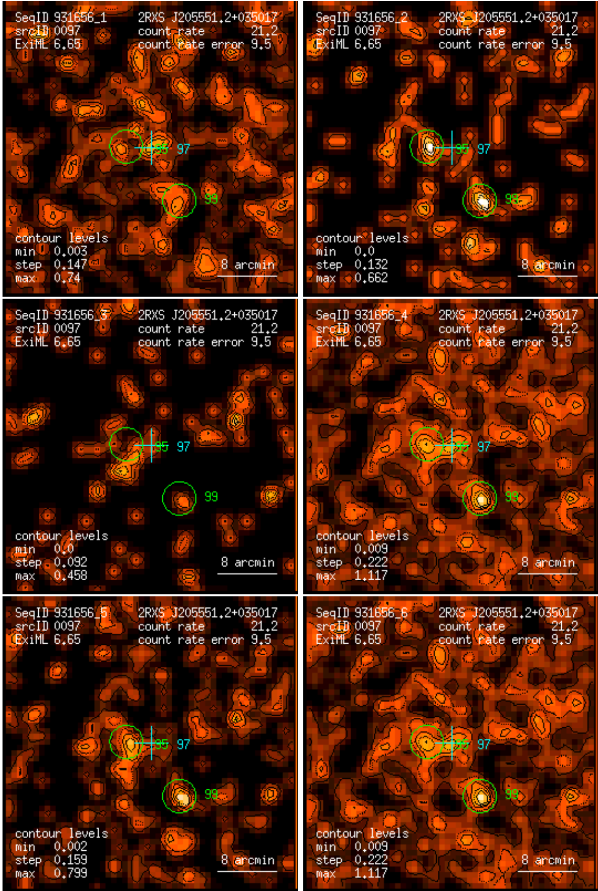
Figure 97: RASS 931656: detection 0097: band rate images, Gaussian filter: (1) PSPC channels 11 – 41, (2) 52 – 90, (3) 91 – 201, (4) 11 – 235, (5) 52 – 201, (6) 11 – 201. Broad band rates in counts/ks. Band rate contour levels in counts/ks/arcmin 2 .
