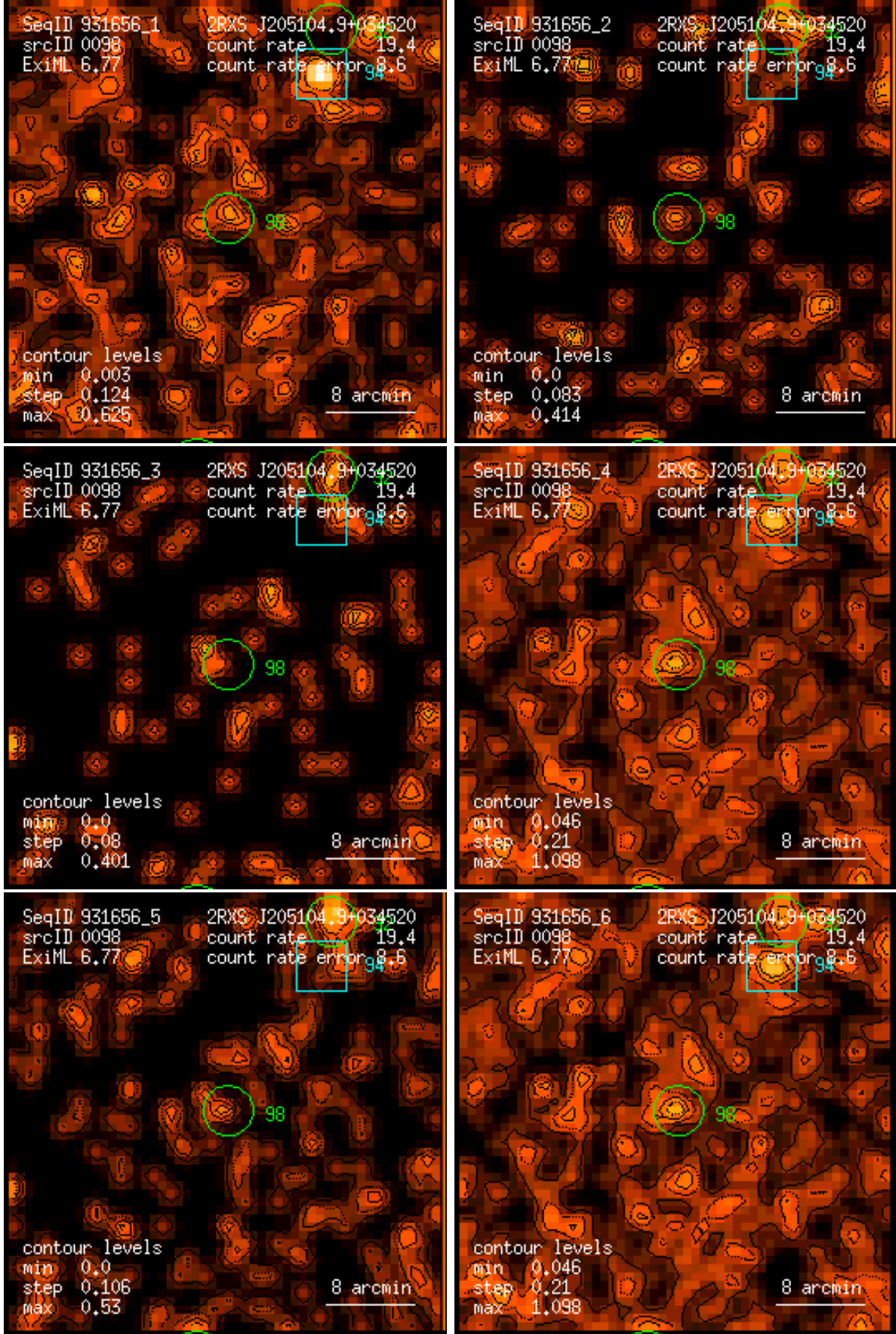
Figure 98: RASS 931656: detection 0098: band rate images, Gaussian filter: (1) PSPC channels 11 – 41, (2) 52 – 90, (3) 91 – 201, (4) 11 – 235, (5) 52 – 201, (6) 11 – 201. Broad band rates in counts/ks. Band rate contour levels in counts/ks/arcmin 2 .
