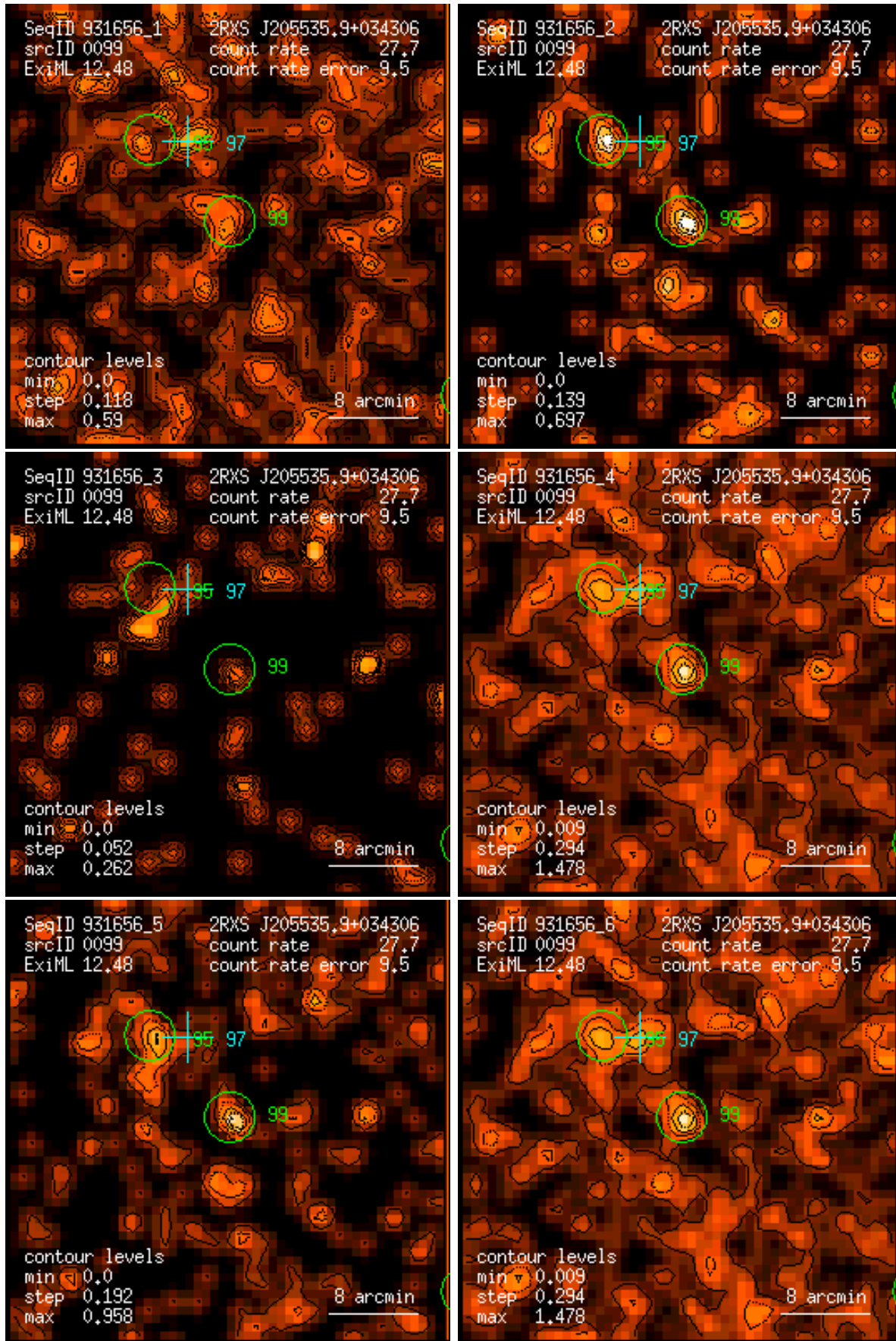
Figure 99: RASS 931656: detection 0099: band rate images, Gaussian filter: (1) PSPC channels 11 – 41, (2) 52 – 90, (3) 91 – 201, (4) 11 – 235, (5) 52 – 201, (6) 11 – 201. Broad band rates in counts/ks. Band rate contour levels in counts/ks/arcmin 2 .
