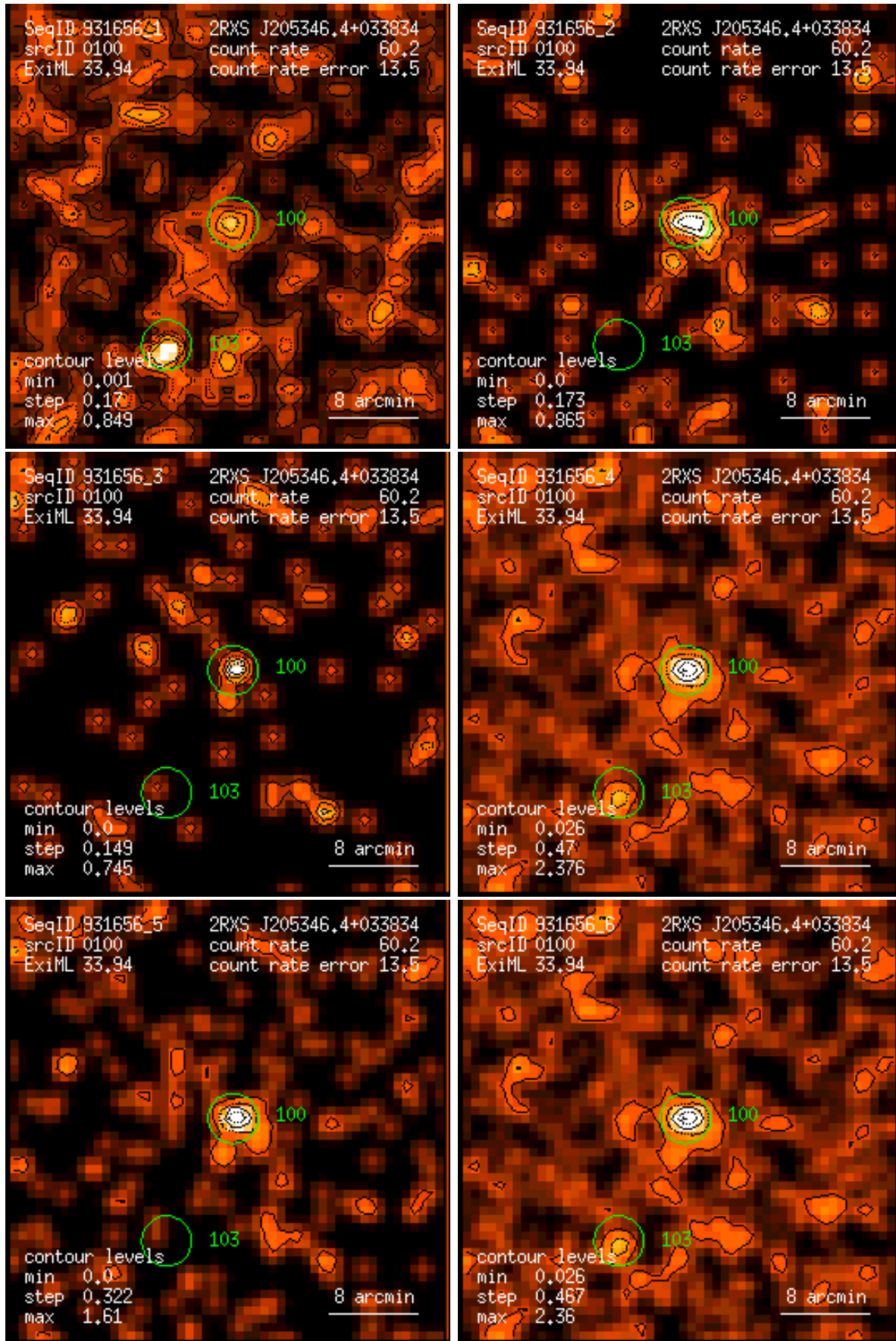
Figure 100: RASS 931656: detection 0100: band rate images, Gaussian filter: (1) PSPC channels 11 – 41, (2) 52 – 90, (3) 91 – 201, (4) 11 – 235, (5) 52 – 201, (6) 11 – 201. Broad band rates in counts/ks. Band rate contour levels in counts/ks/arcmin 2 .
