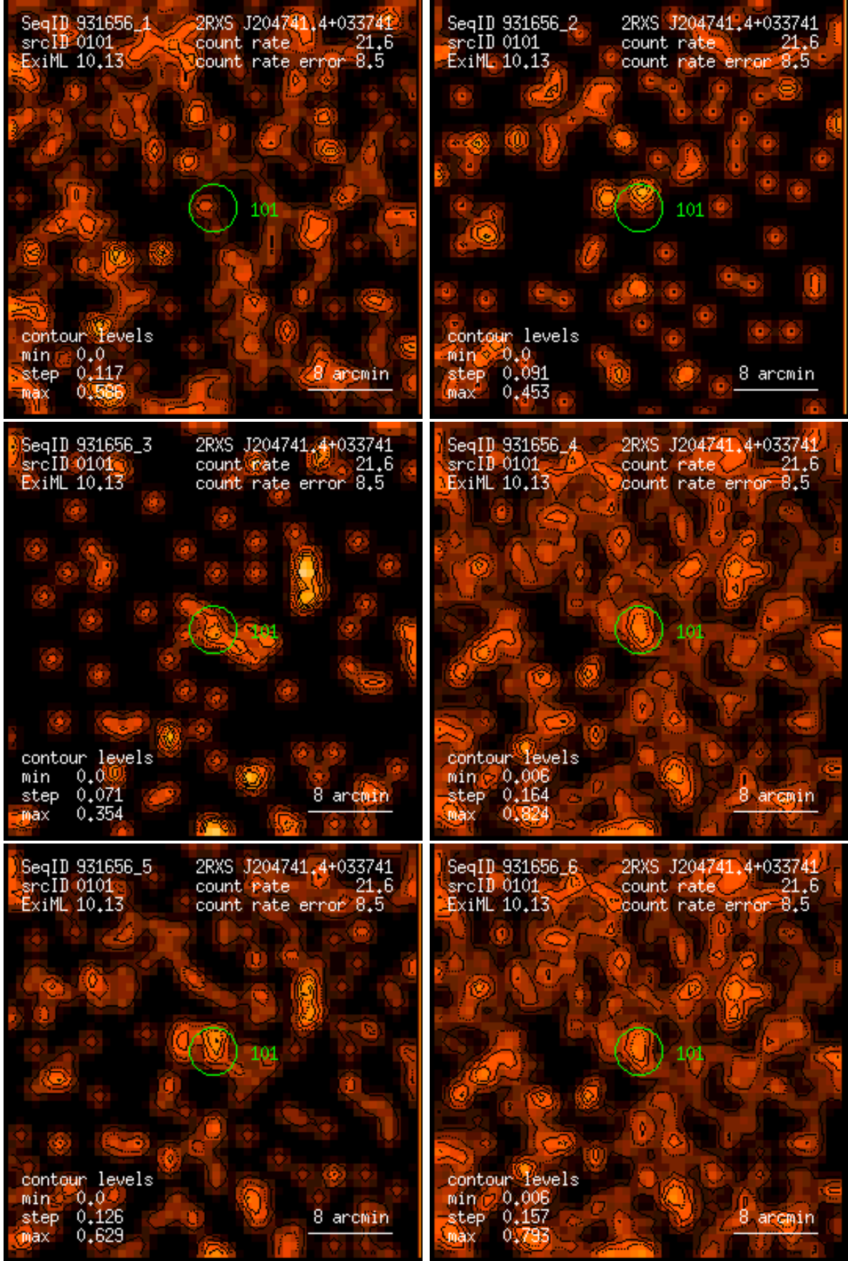
Figure 101: RASS 931656: detection 0101: band rate images, Gaussian filter: (1) PSPC channels 11 – 41, (2) 52 – 90, (3) 91 – 201, (4) 11 – 235, (5) 52 – 201, (6) 11 – 201. Broad band rates in counts/ks. Band rate contour levels in counts/ks/arcmin 2 .
