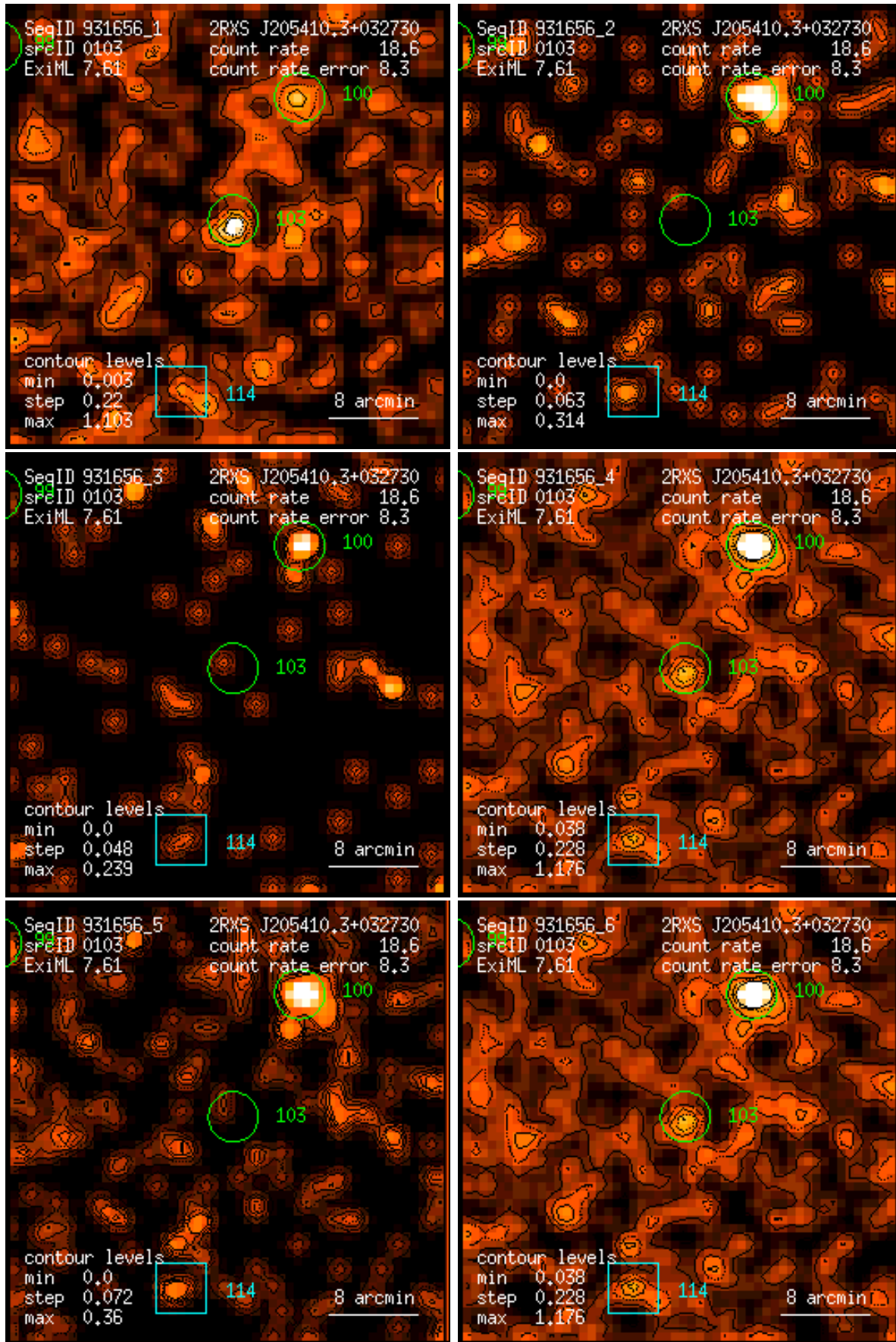
Figure 103: RASS 931656: detection 0103: band rate images, Gaussian filter: (1) PSPC channels 11 – 41, (2) 52 – 90, (3) 91 – 201, (4) 11 – 235, (5) 52 – 201, (6) 11 – 201. Broad band rates in counts/ks. Band rate contour levels in counts/ks/arcmin 2 .
