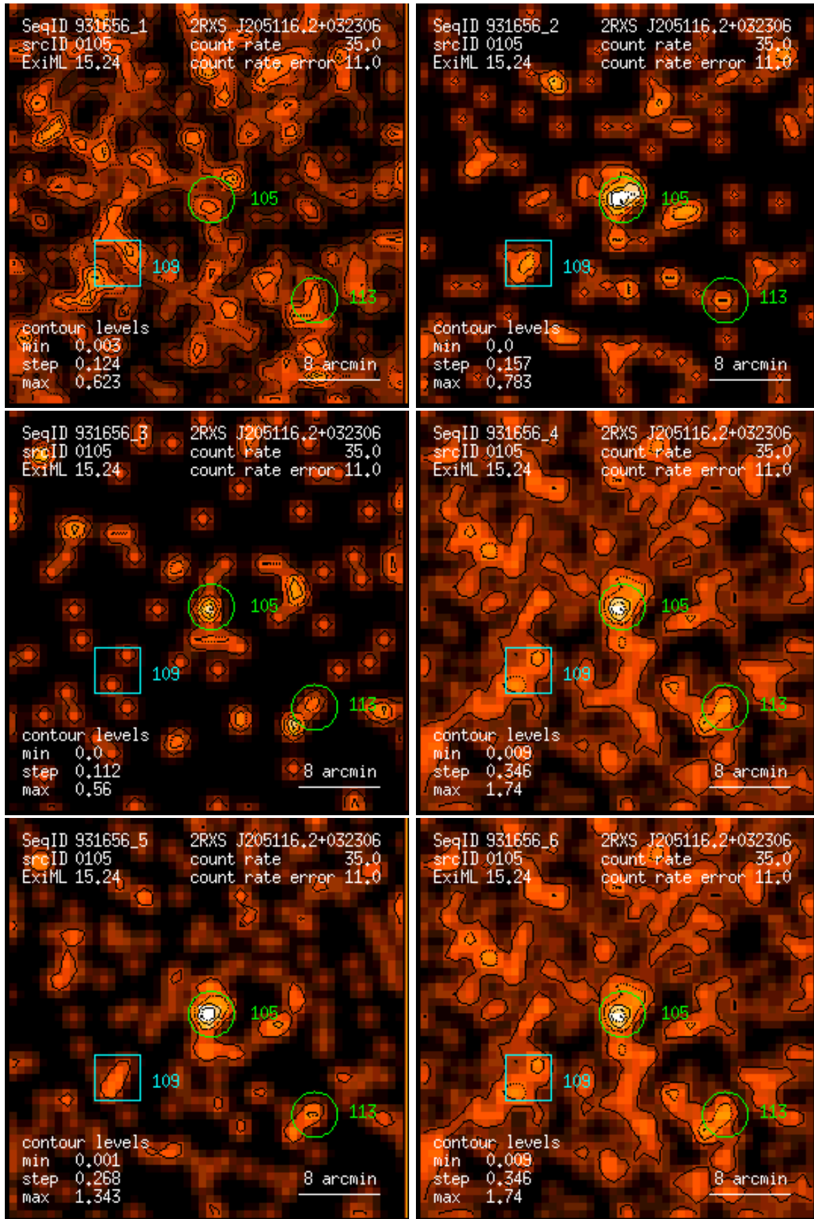
Figure 105: RASS 931656: detection 0105: band rate images, Gaussian filter: (1) PSPC channels 11 – 41, (2) 52 – 90, (3) 91 – 201, (4) 11 – 235, (5) 52 – 201, (6) 11 – 201. Broad band rates in counts/ks. Band rate contour levels in counts/ks/arcmin 2 .
