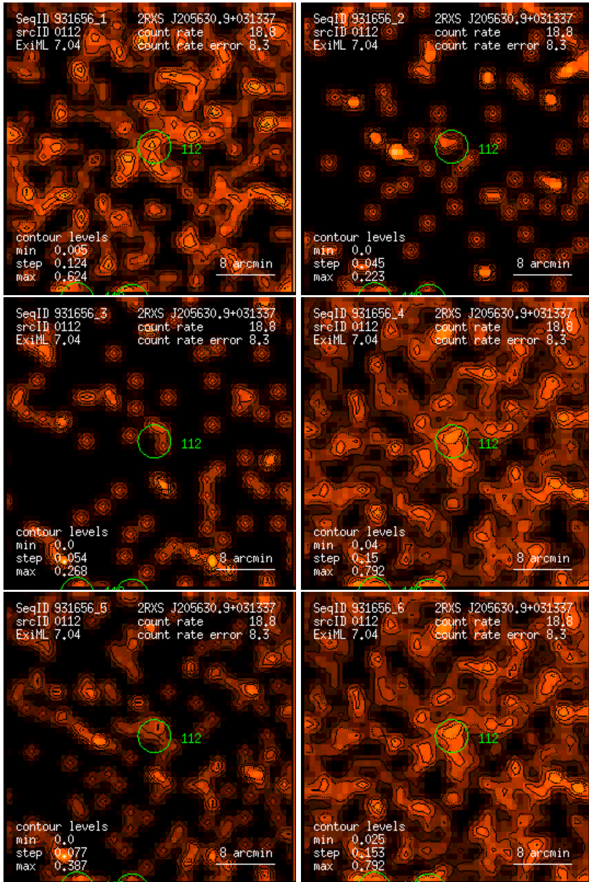
Figure 112: RASS 931656: detection 0112: band rate images, Gaussian filter: (1) PSPC channels 11 – 41, (2) 52 – 90, (3) 91 – 201, (4) 11 – 235, (5) 52 – 201, (6) 11 – 201. Broad band rates in counts/ks. Band rate contour levels in counts/ks/arcmin 2 .
