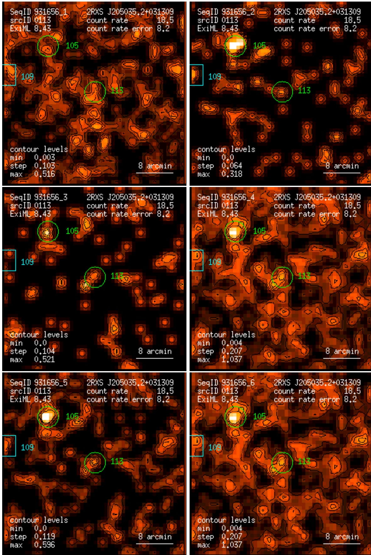
Figure 113: RASS 931656: detection 0113: band rate images, Gaussian filter: (1) PSPC channels 11 – 41, (2) 52 – 90, (3) 91 – 201, (4) 11 – 235, (5) 52 – 201, (6) 11 – 201. Broad band rates in counts/ks. Band rate contour levels in counts/ks/arcmin 2 .
