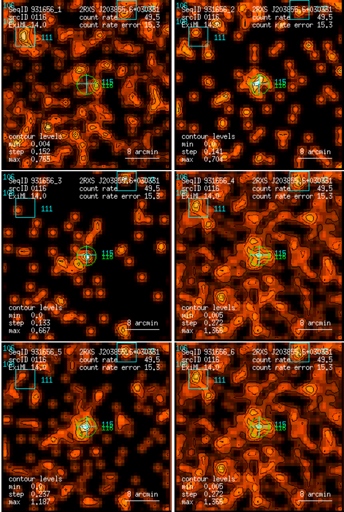
Figure 116: RASS 931656: detection 0116: band rate images, Gaussian filter: (1) PSPC channels 11 – 41, (2) 52 – 90, (3) 91 – 201, (4) 11 – 235, (5) 52 – 201, (6) 11 – 201. Broad band rates in counts/ks. Band rate contour levels in counts/ks/arcmin 2 .
