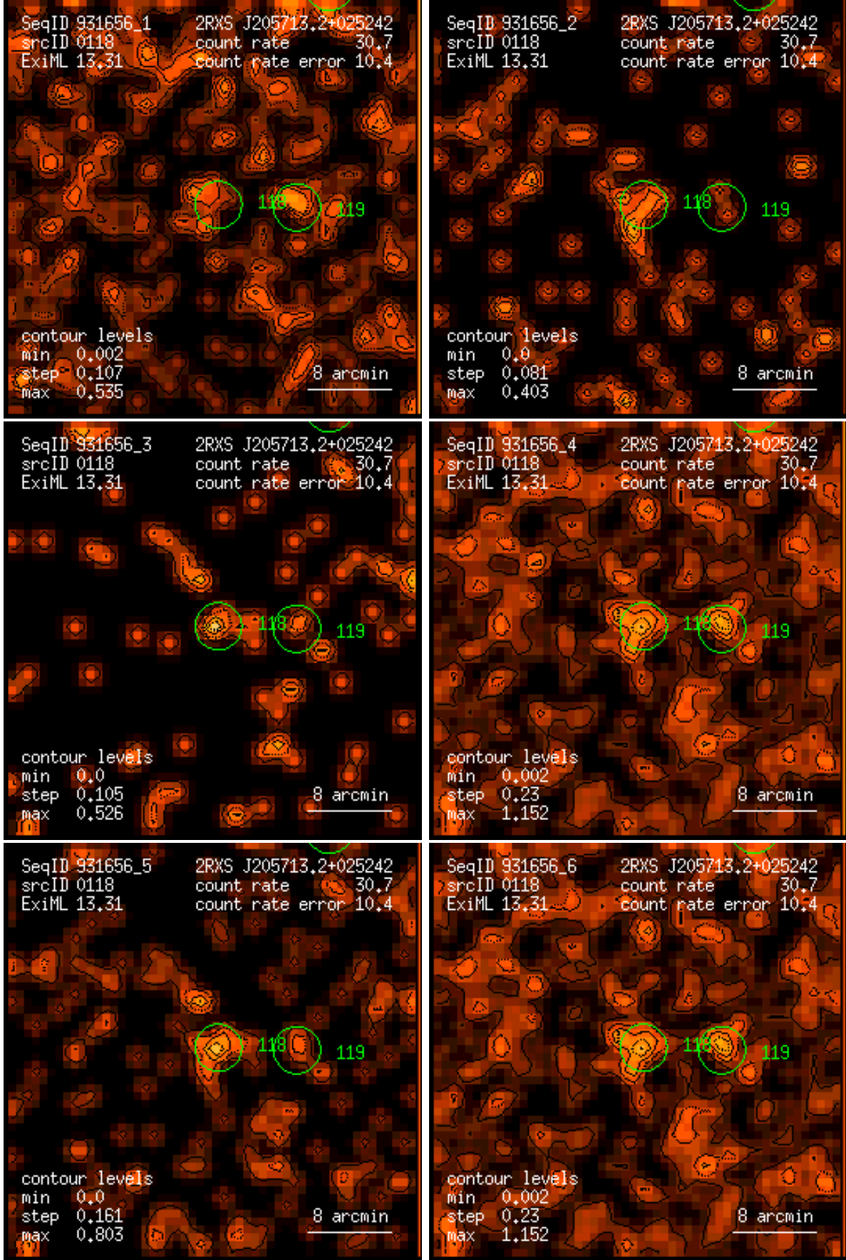
Figure 118: RASS 931656: detection 0118: band rate images, Gaussian filter: (1) PSPC channels 11 – 41, (2) 52 – 90, (3) 91 – 201, (4) 11 – 235, (5) 52 – 201, (6) 11 – 201. Broad band rates in counts/ks. Band rate contour levels in counts/ks/arcmin 2 .
