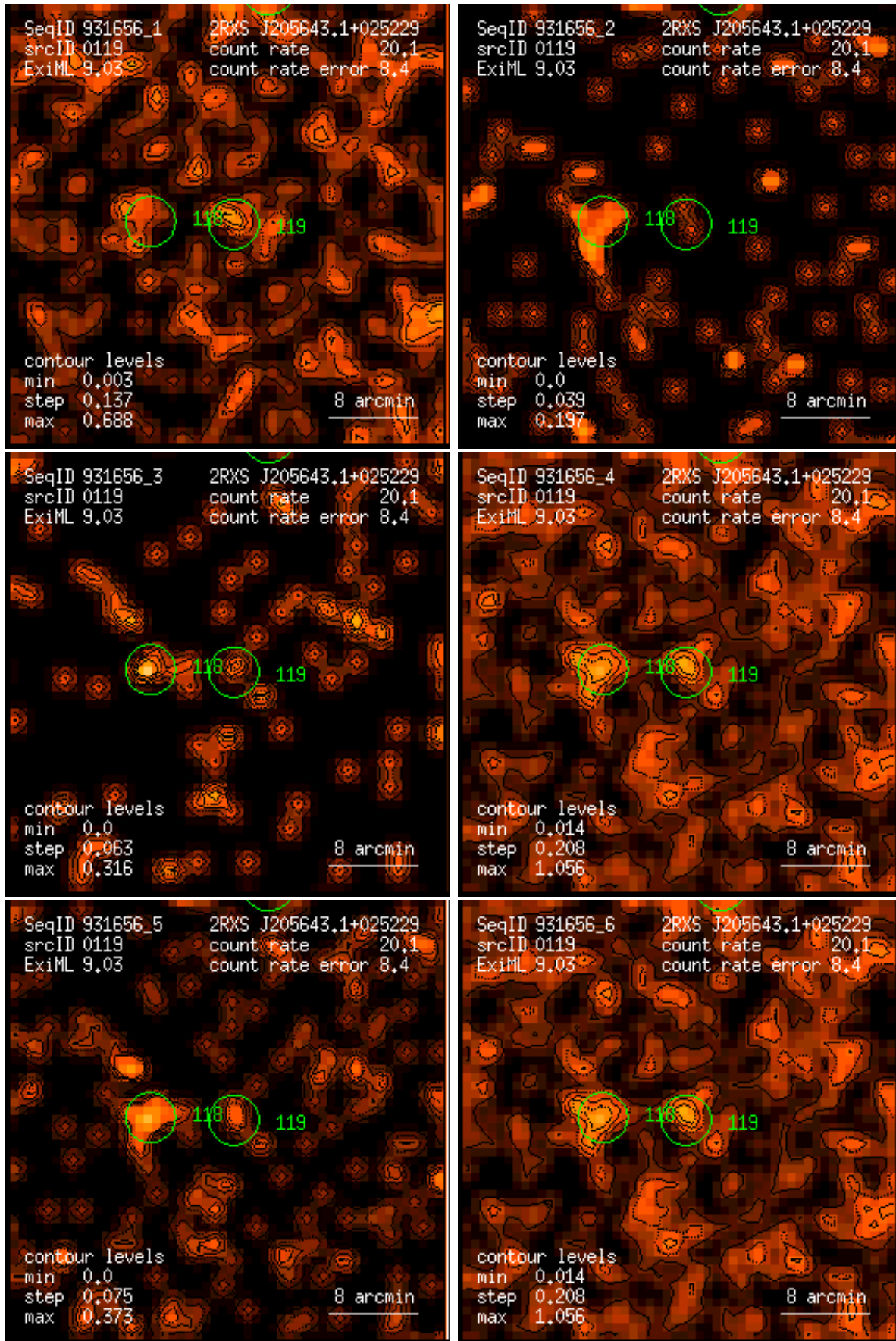
Figure 119: RASS 931656: detection 0119: band rate images, Gaussian filter: (1) PSPC channels 11 – 41, (2) 52 – 90, (3) 91 – 201, (4) 11 – 235, (5) 52 – 201, (6) 11 – 201. Broad band rates in counts/ks. Band rate contour levels in counts/ks/arcmin 2 .
