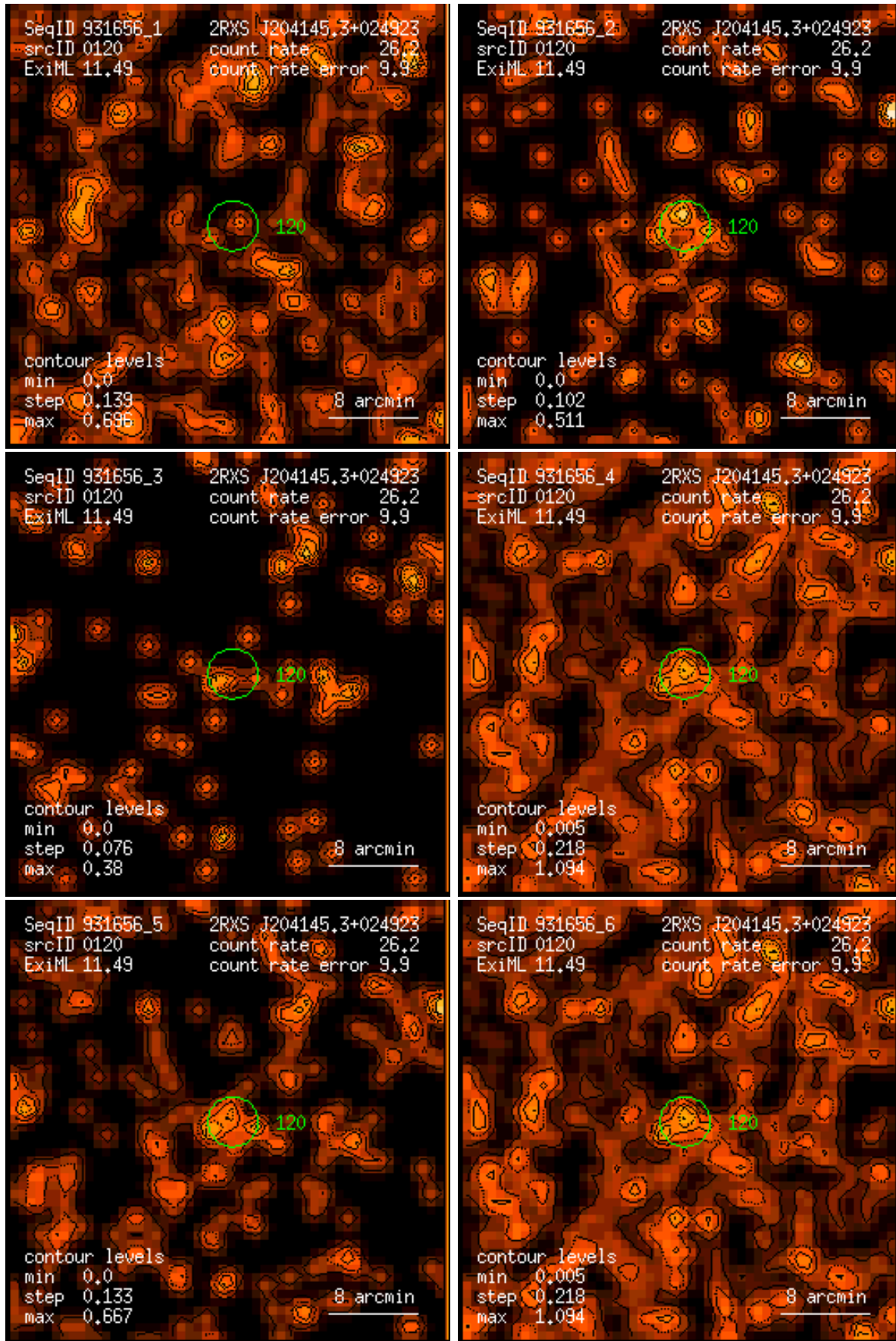
Figure 120: RASS 931656: detection 0120: band rate images, Gaussian filter: (1) PSPC channels 11 – 41, (2) 52 – 90, (3) 91 – 201, (4) 11 – 235, (5) 52 – 201, (6) 11 – 201. Broad band rates in counts/ks. Band rate contour levels in counts/ks/arcmin 2 .
