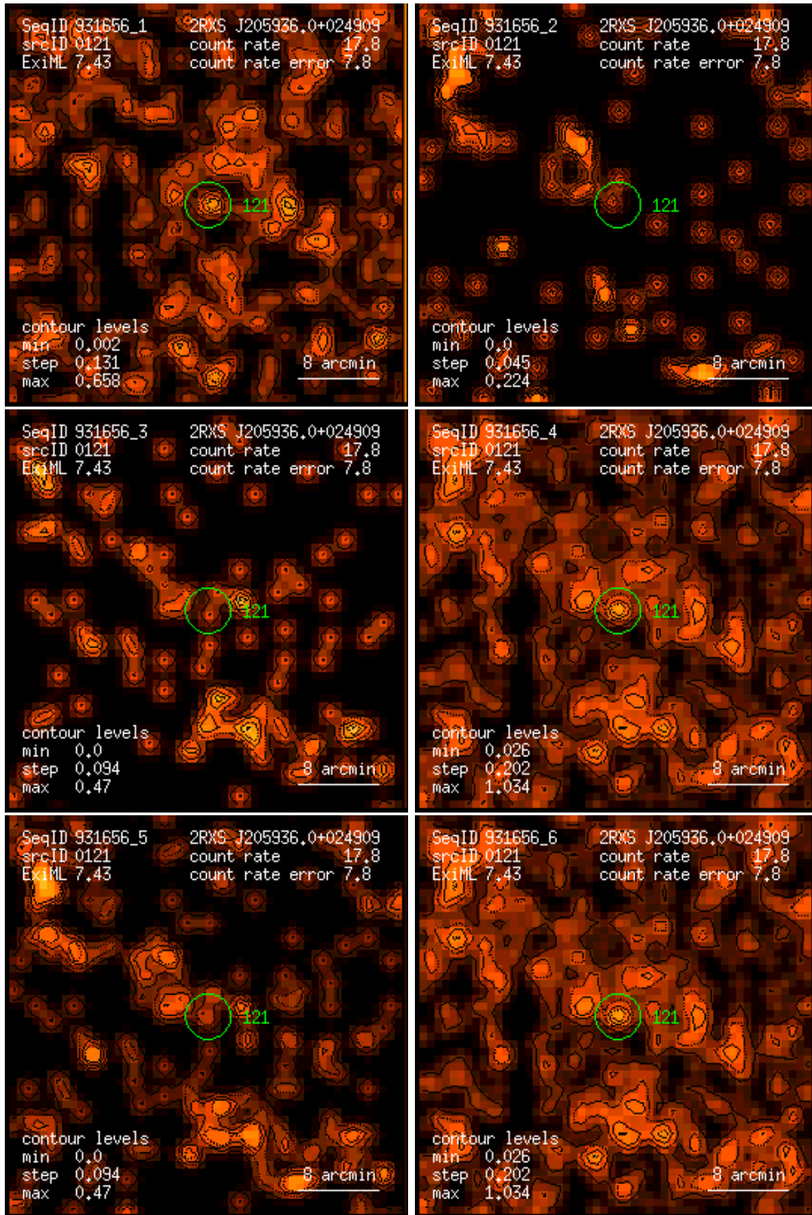
Figure 121: RASS 931656: detection 0121: band rate images, Gaussian filter: (1) PSPC channels 11 – 41, (2) 52 – 90, (3) 91 – 201, (4) 11 – 235, (5) 52 – 201, (6) 11 – 201. Broad band rates in counts/ks. Band rate contour levels in counts/ks/arcmin 2 .
