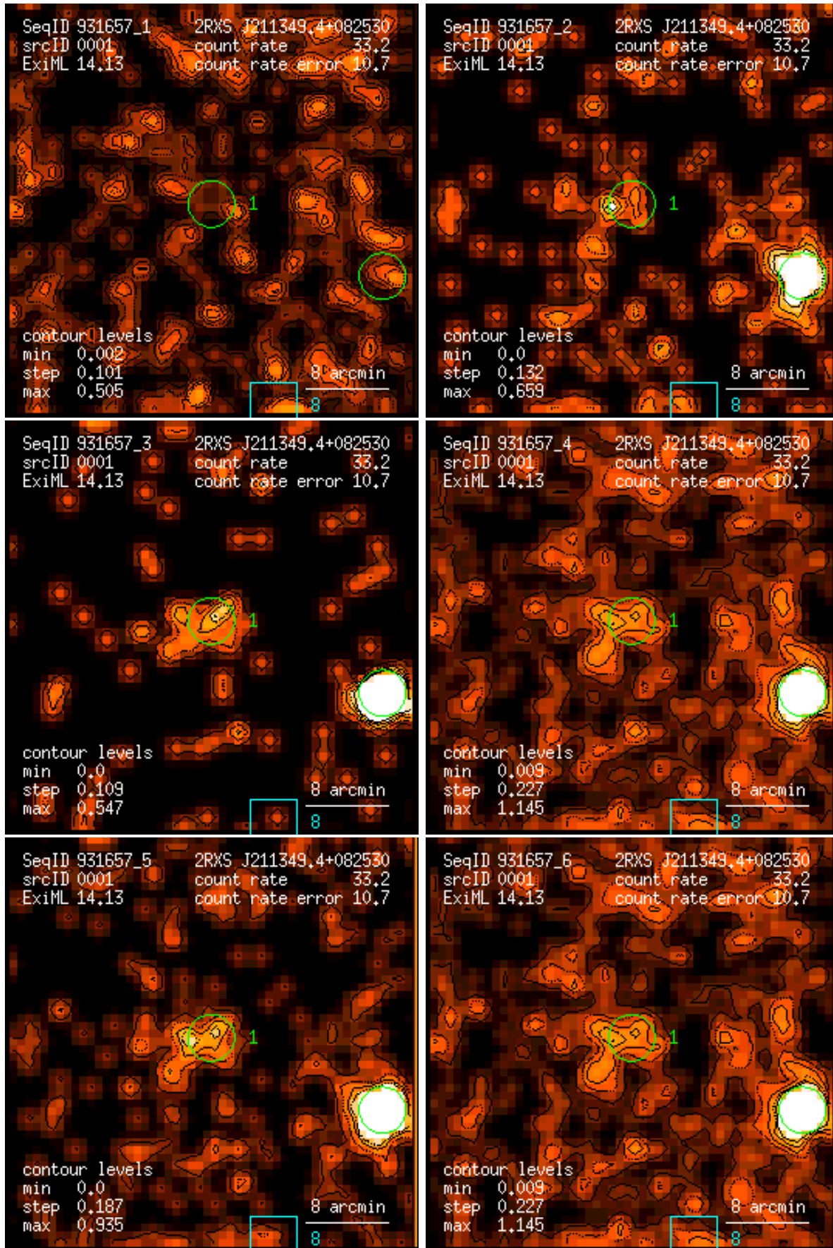
Figure 1: RASS 931657: detection 0001: band rate images, Gaussian filter: (1) PSPC channels 11 – 41, (2) 52 – 90, (3) 91 – 201, (4) 11 – 235, (5) 52 – 201, (6) 11 – 201. Broad band rates in counts/ks. Band rate contour levels in counts/ks/arcmin 2 .
