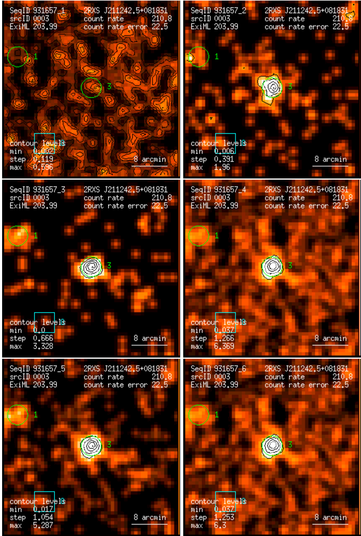
Figure 3: RASS 931657: detection 0003: band rate images, Gaussian filter: (1) PSPC channels 11 – 41, (2) 52 – 90, (3) 91 – 201, (4) 11 – 235, (5) 52 – 201, (6) 11 – 201. Broad band rates in counts/ks. Band rate contour levels in counts/ks/arcmin 2 .
