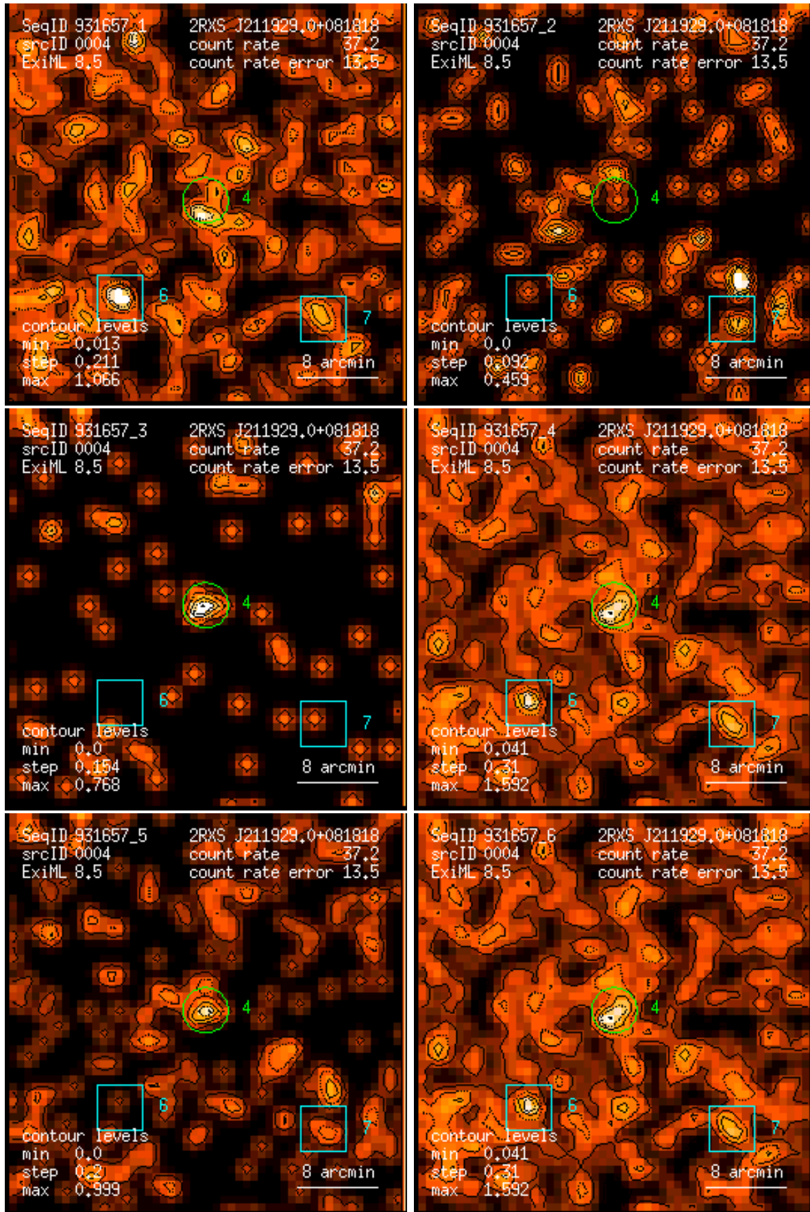
Figure 4: RASS 931657: detection 0004: band rate images, Gaussian filter: (1) PSPC channels 11 – 41, (2) 52 – 90, (3) 91 – 201, (4) 11 – 235, (5) 52 – 201, (6) 11 – 201. Broad band rates in counts/ks. Band rate contour levels in counts/ks/arcmin 2 .
