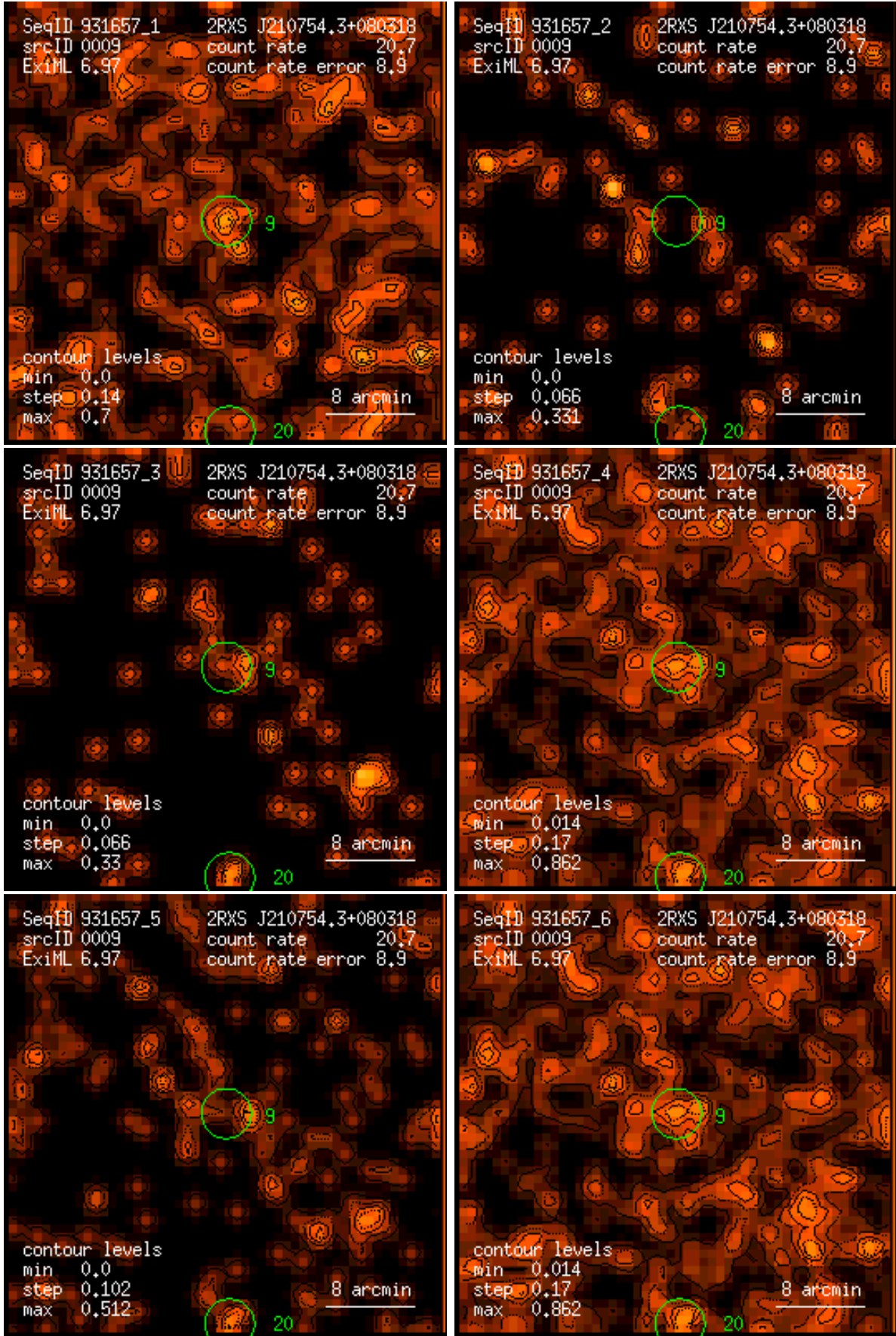
Figure 9: RASS 931657: detection 0009: band rate images, Gaussian filter: (1) PSPC channels 11 – 41, (2) 52 – 90, (3) 91 – 201, (4) 11 – 235, (5) 52 – 201, (6) 11 – 201. Broad band rates in counts/ks. Band rate contour levels in counts/ks/arcmin 2 .
