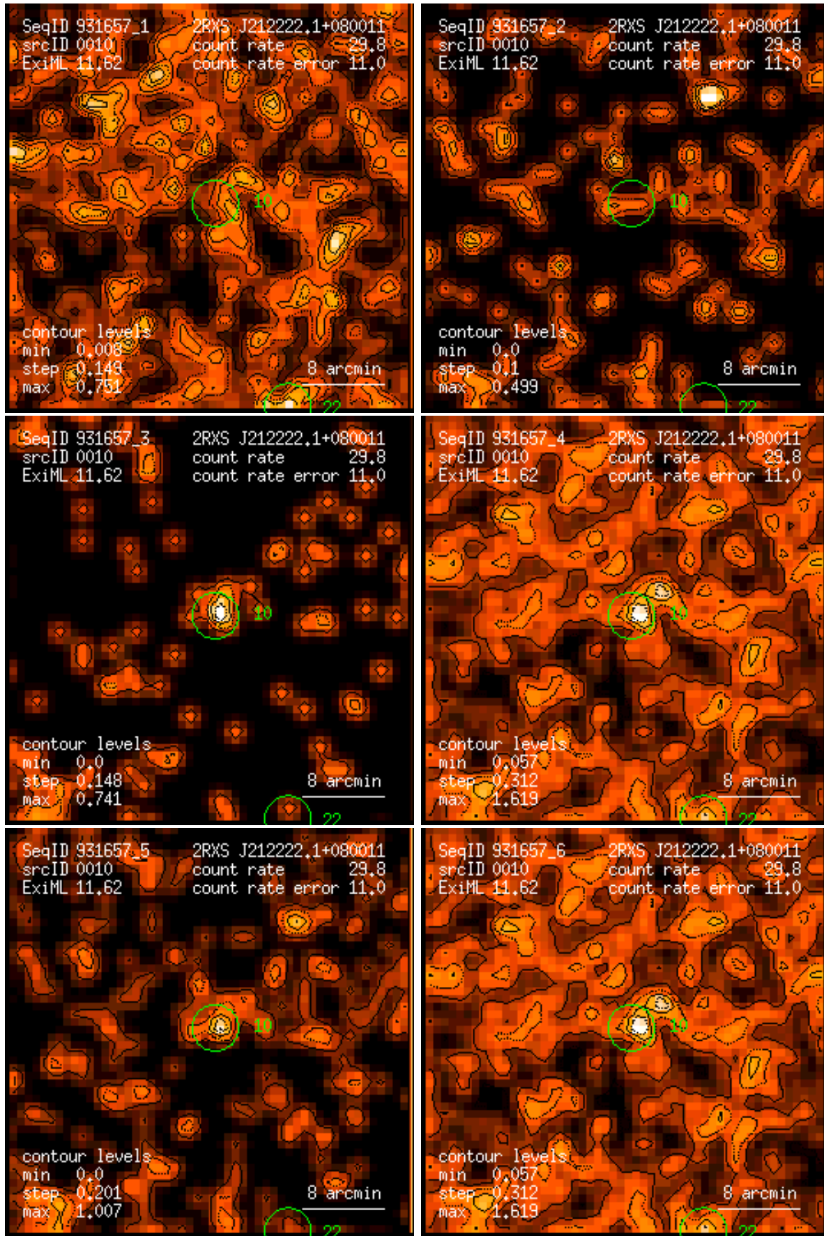
Figure 10: RASS 931657: detection 0010: band rate images, Gaussian filter: (1) PSPC channels 11 – 41, (2) 52 – 90, (3) 91 – 201, (4) 11 – 235, (5) 52 – 201, (6) 11 – 201. Broad band rates in counts/ks. Band rate contour levels in counts/ks/arcmin 2 .
