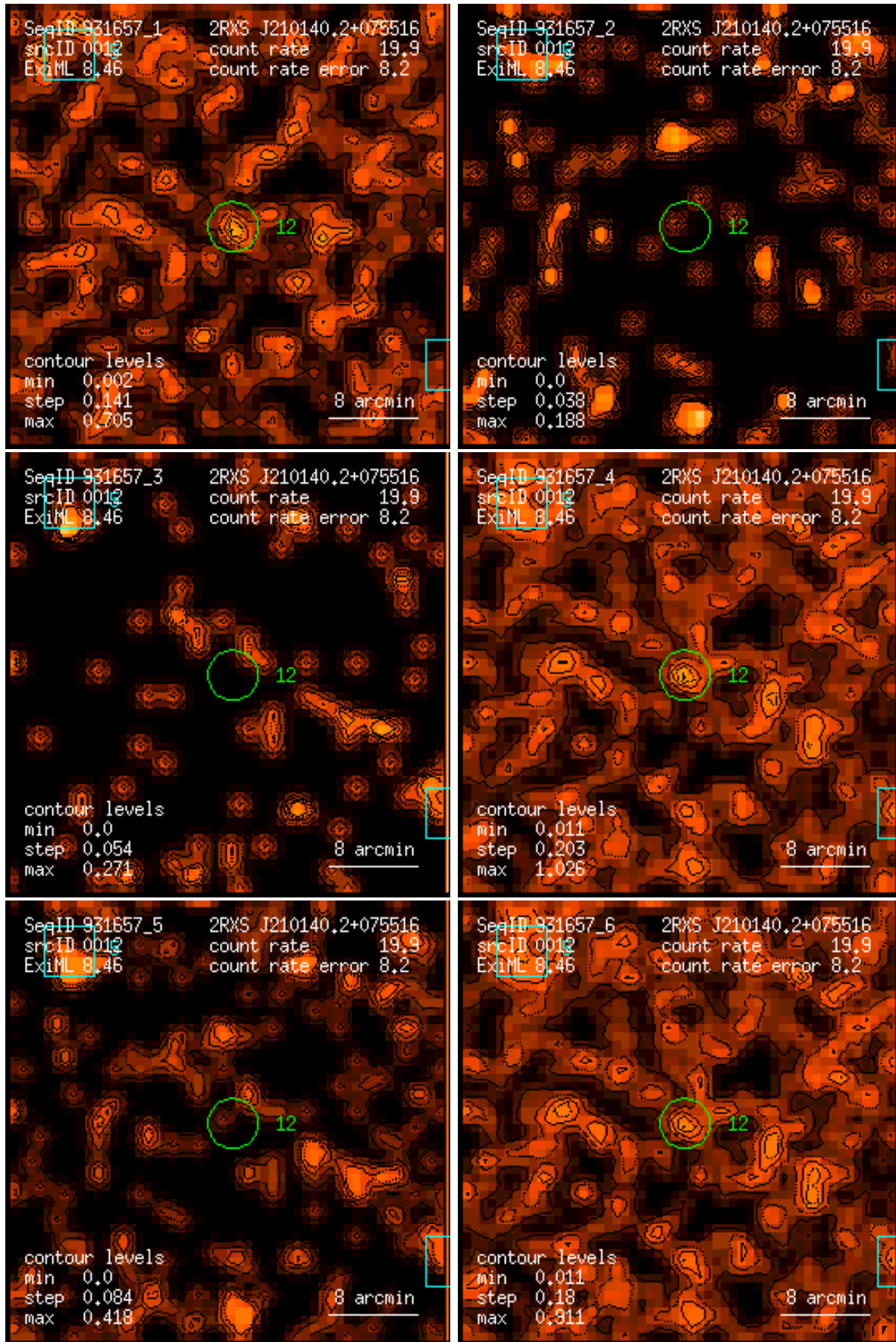
Figure 12: RASS 931657: detection 0012: band rate images, Gaussian filter: (1) PSPC channels 11 – 41, (2) 52 – 90, (3) 91 – 201, (4) 11 – 235, (5) 52 – 201, (6) 11 – 201. Broad band rates in counts/ks. Band rate contour levels in counts/ks/arcmin 2 .
