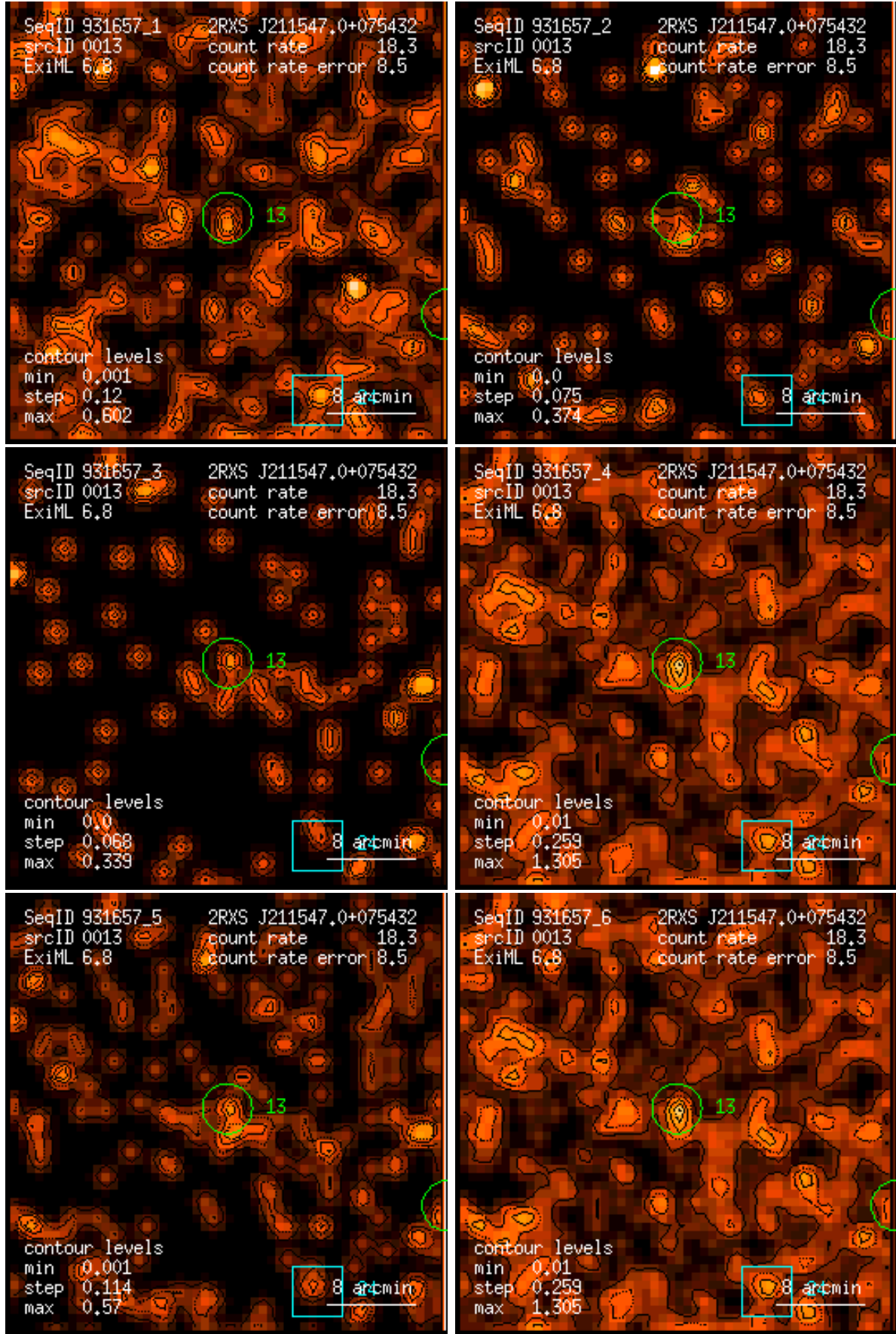
Figure 13: RASS 931657: detection 0013: band rate images, Gaussian filter: (1) PSPC channels 11 – 41, (2) 52 – 90, (3) 91 – 201, (4) 11 – 235, (5) 52 – 201, (6) 11 – 201. Broad band rates in counts/ks. Band rate contour levels in counts/ks/arcmin 2 .
