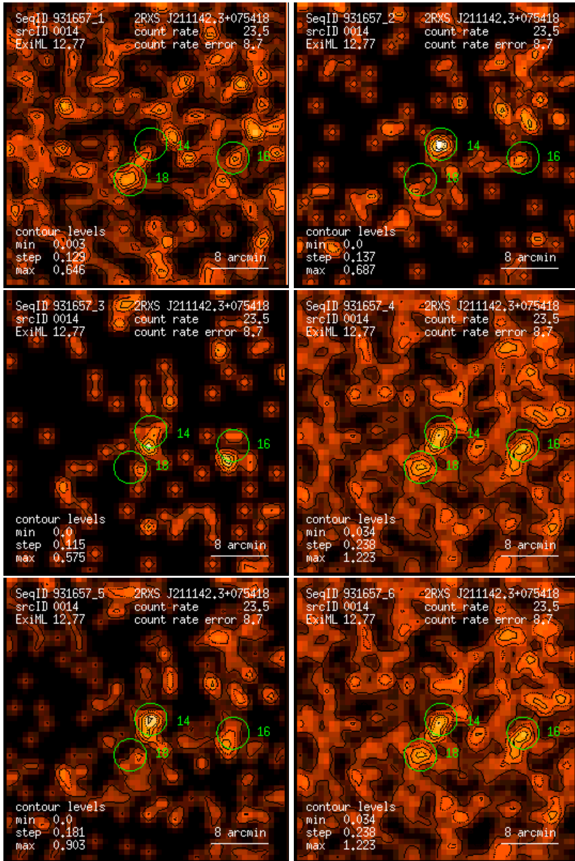
Figure 14: RASS 931657: detection 0014: band rate images, Gaussian filter: (1) PSPC channels 11 – 41, (2) 52 – 90, (3) 91 – 201, (4) 11 – 235, (5) 52 – 201, (6) 11 – 201. Broad band rates in counts/ks. Band rate contour levels in counts/ks/arcmin 2 .
