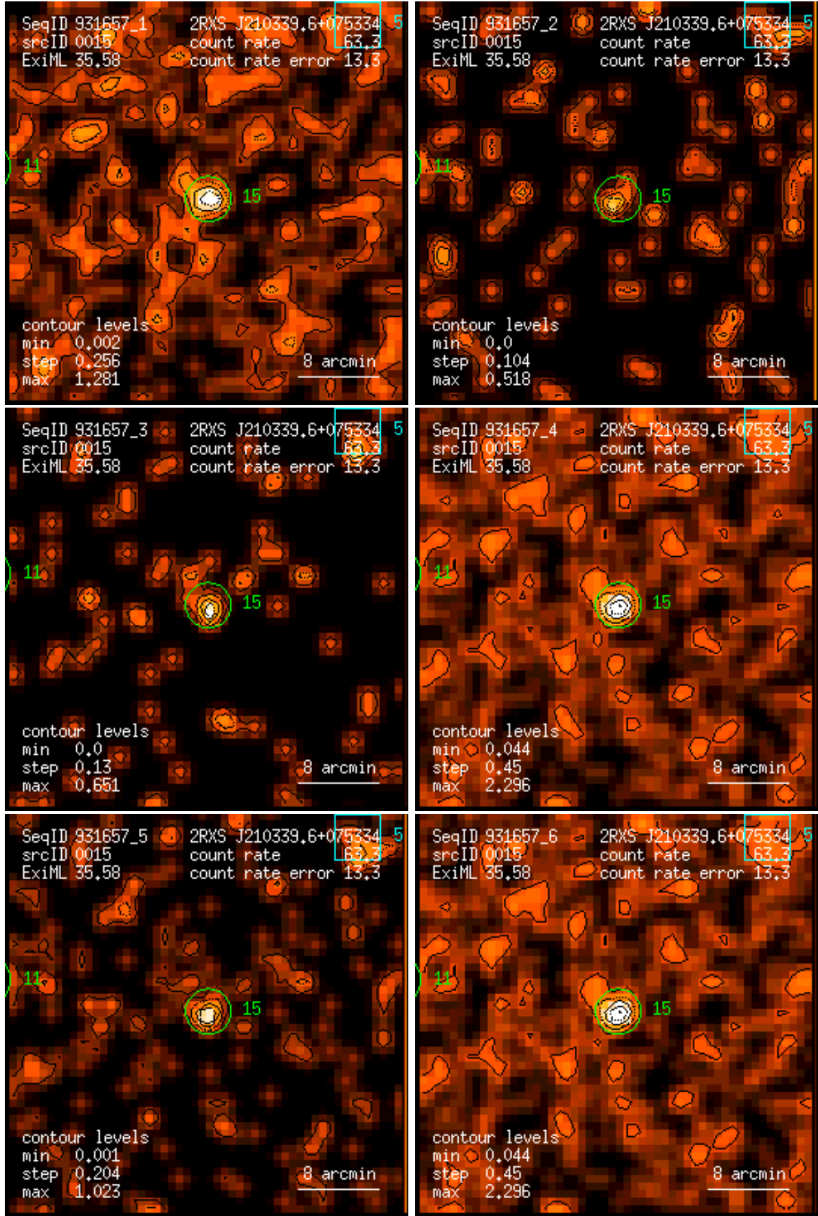
Figure 15: RASS 931657: detection 0015: band rate images, Gaussian filter: (1) PSPC channels 11 – 41, (2) 52 – 90, (3) 91 – 201, (4) 11 – 235, (5) 52 – 201, (6) 11 – 201. Broad band rates in counts/ks. Band rate contour levels in counts/ks/arcmin 2 .
