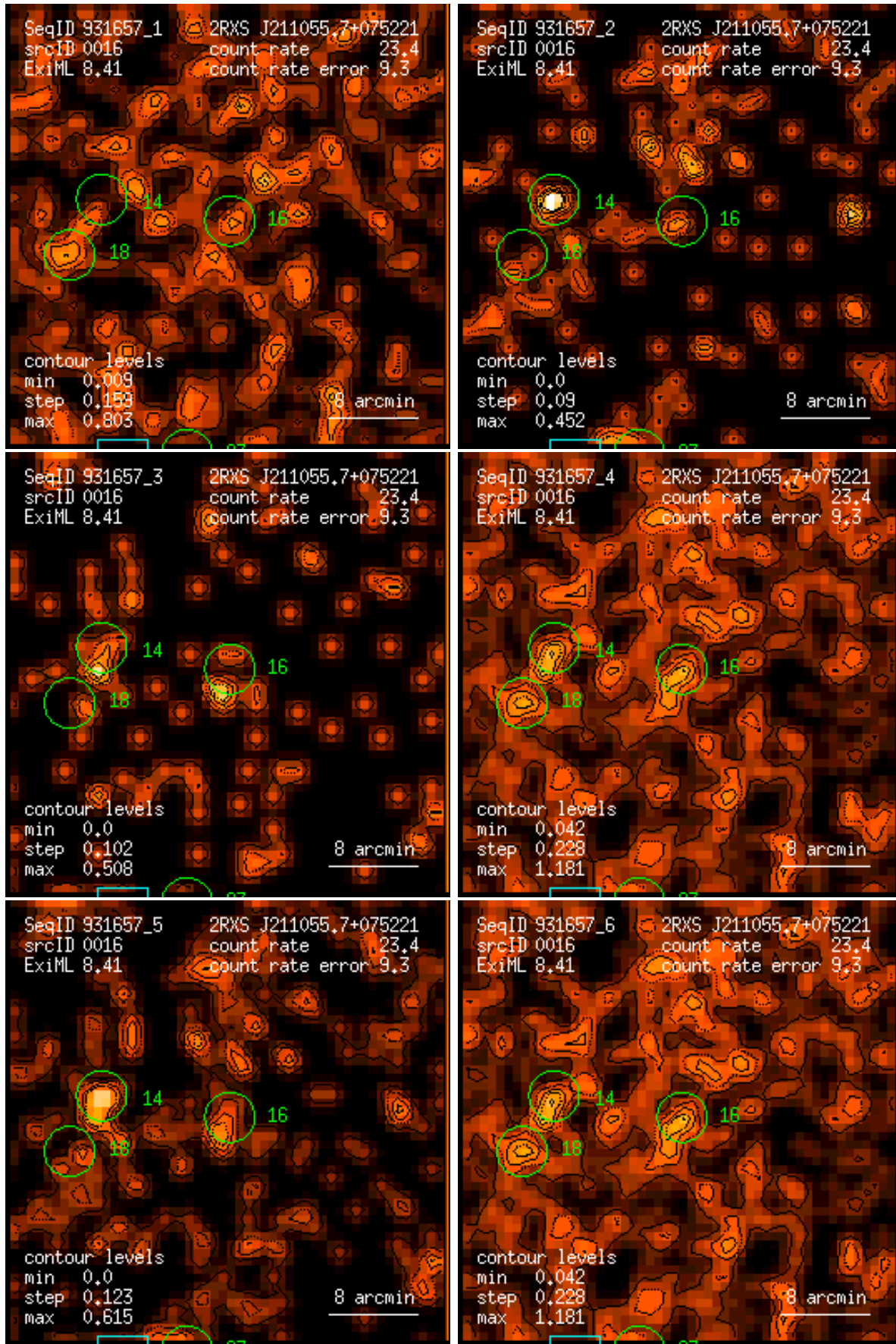
Figure 16: RASS 931657: detection 0016: band rate images, Gaussian filter: (1) PSPC channels 11 – 41, (2) 52 – 90, (3) 91 – 201, (4) 11 – 235, (5) 52 – 201, (6) 11 – 201. Broad band rates in counts/ks. Band rate contour levels in counts/ks/arcmin 2 .
