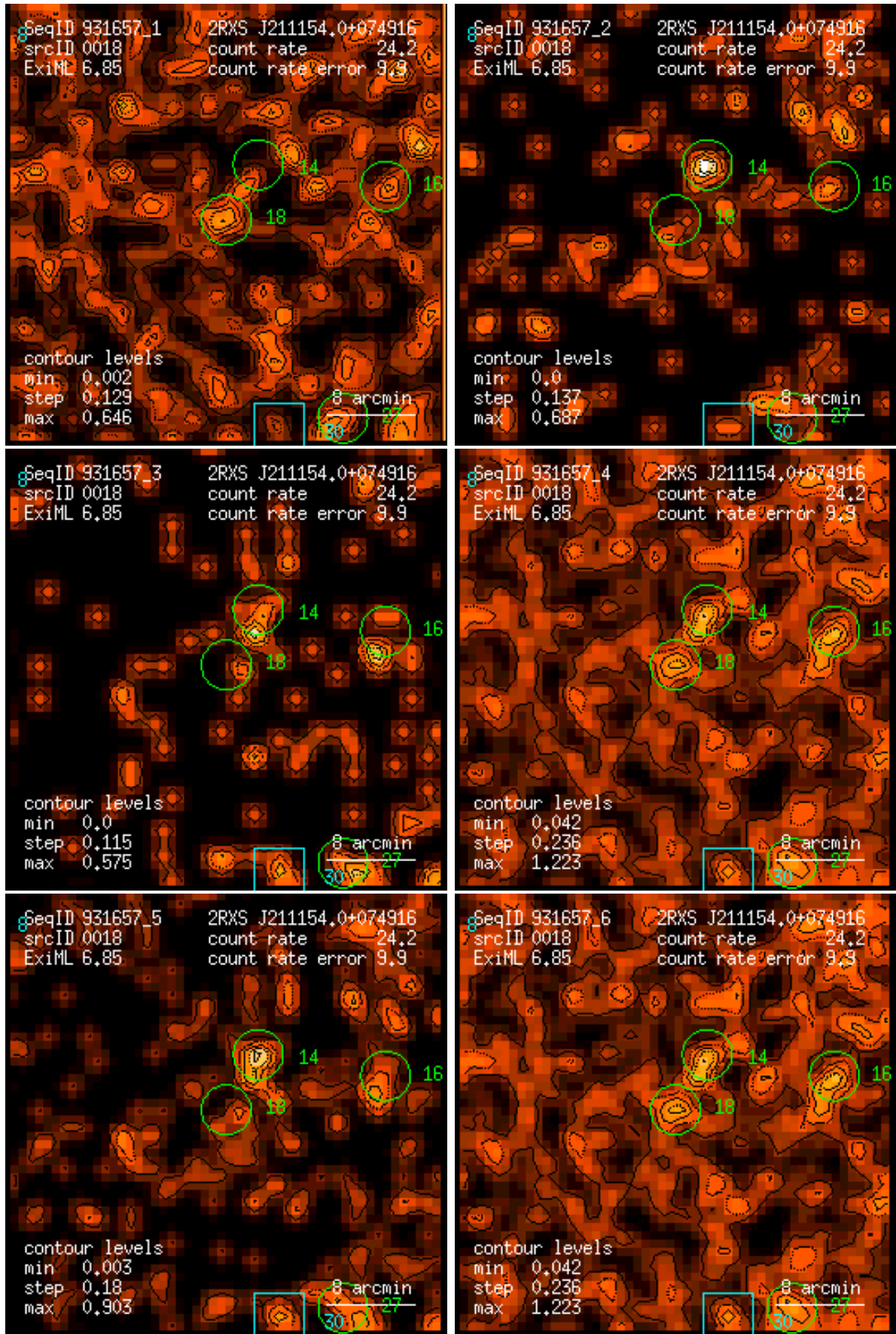
Figure 18: RASS 931657: detection 0018: band rate images, Gaussian filter: (1) PSPC channels 11 – 41, (2) 52 – 90, (3) 91 – 201, (4) 11 – 235, (5) 52 – 201, (6) 11 – 201. Broad band rates in counts/ks. Band rate contour levels in counts/ks/arcmin 2 .
