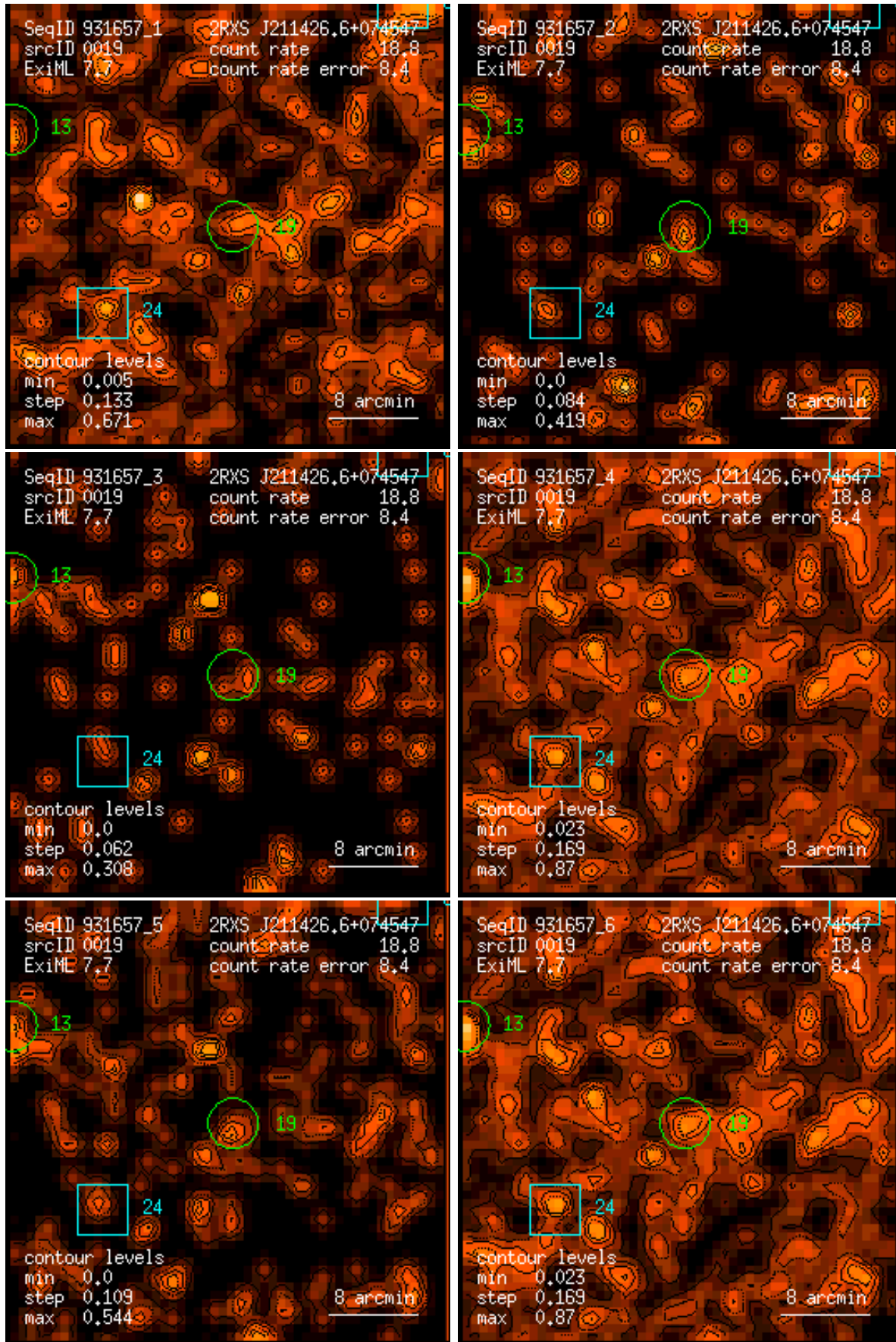
Figure 19: RASS 931657: detection 0019: band rate images, Gaussian filter: (1) PSPC channels 11 – 41, (2) 52 – 90, (3) 91 – 201, (4) 11 – 235, (5) 52 – 201, (6) 11 – 201. Broad band rates in counts/ks. Band rate contour levels in counts/ks/arcmin 2 .
