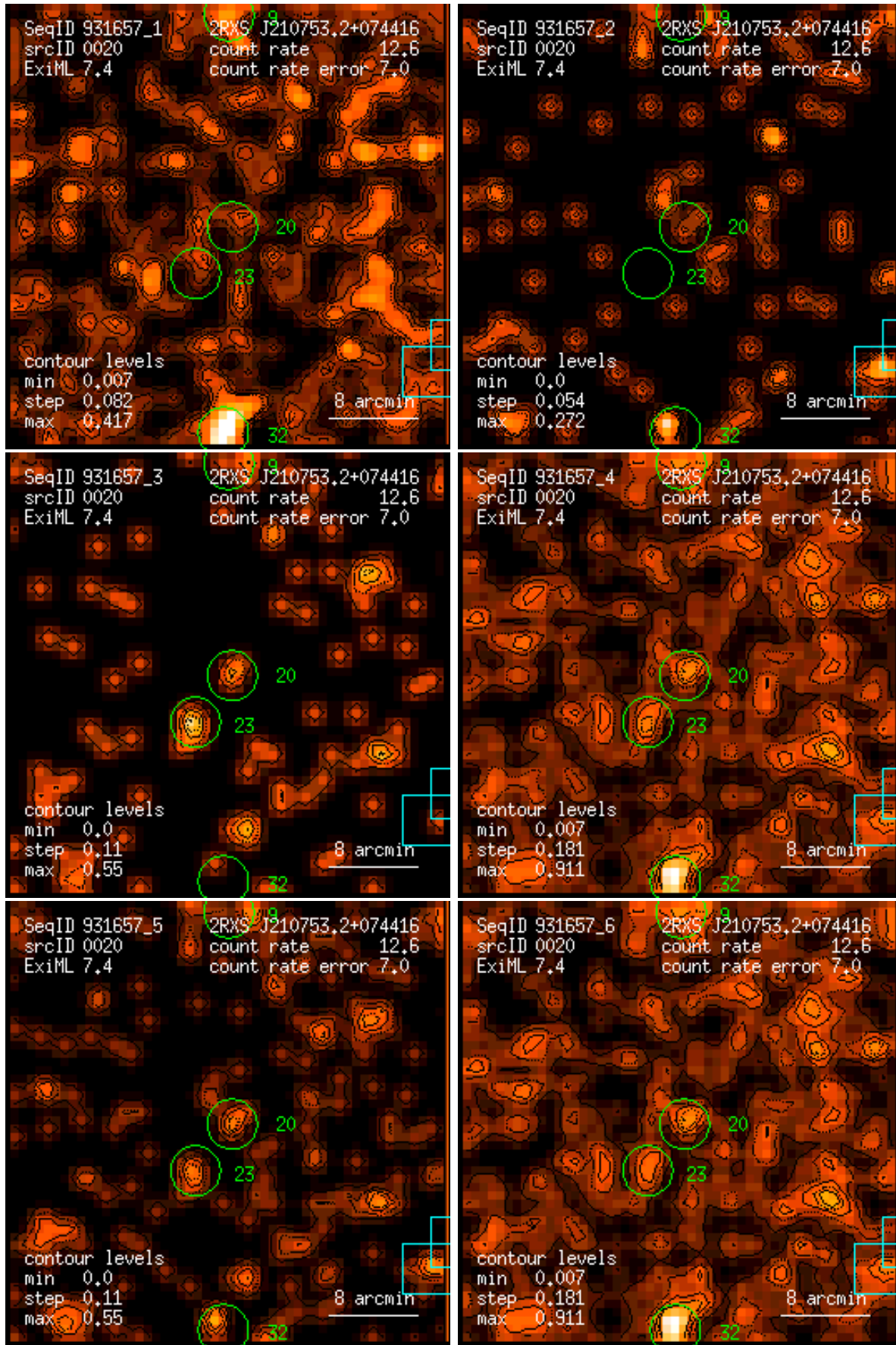
Figure 20: RASS 931657: detection 0020: band rate images, Gaussian filter: (1) PSPC channels 11 – 41, (2) 52 – 90, (3) 91 – 201, (4) 11 – 235, (5) 52 – 201, (6) 11 – 201. Broad band rates in counts/ks. Band rate contour levels in counts/ks/arcmin 2 .
