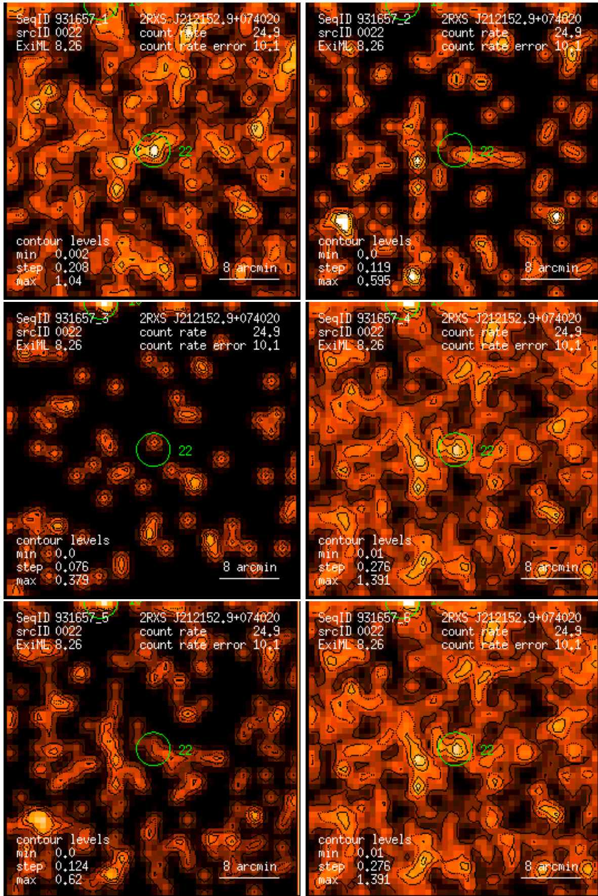
Figure 22: RASS 931657: detection 0022: band rate images, Gaussian filter: (1) PSPC channels 11 – 41, (2) 52 – 90, (3) 91 – 201, (4) 11 – 235, (5) 52 – 201, (6) 11 – 201. Broad band rates in counts/ks. Band rate contour levels in counts/ks/arcmin 2 .
