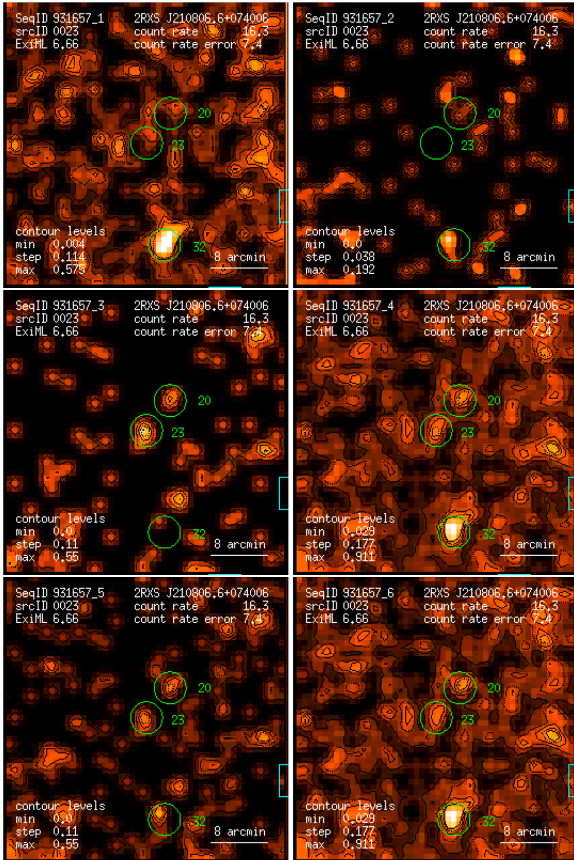
Figure 23: RASS 931657: detection 0023: band rate images, Gaussian filter: (1) PSPC channels 11 – 41, (2) 52 – 90, (3) 91 – 201, (4) 11 – 235, (5) 52 – 201, (6) 11 – 201. Broad band rates in counts/ks. Band rate contour levels in counts/ks/arcmin 2 .
