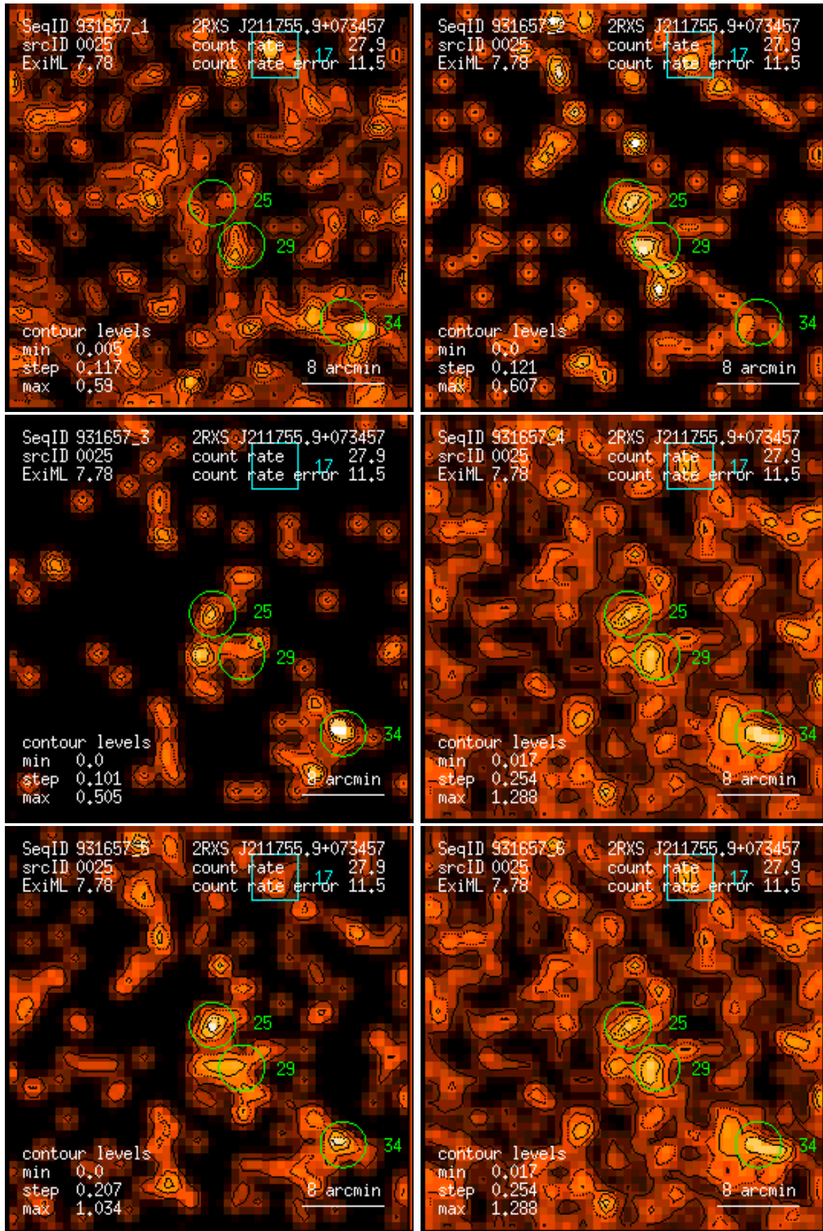
Figure 25: RASS 931657: detection 0025: band rate images, Gaussian filter: (1) PSPC channels 11 – 41, (2) 52 – 90, (3) 91 – 201, (4) 11 – 235, (5) 52 – 201, (6) 11 – 201. Broad band rates in counts/ks. Band rate contour levels in counts/ks/arcmin 2 .
