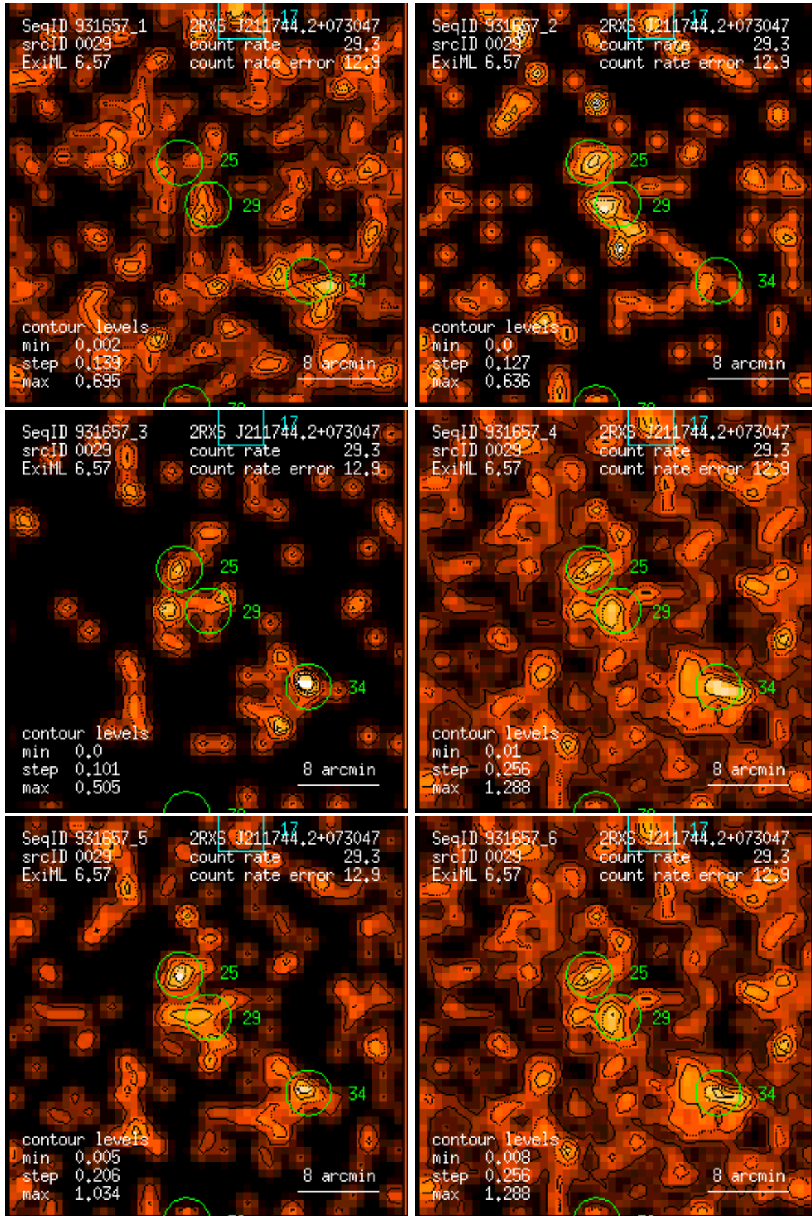
Figure 29: RASS 931657: detection 0029: band rate images, Gaussian filter: (1) PSPC channels 11 – 41, (2) 52 – 90, (3) 91 – 201, (4) 11 – 235, (5) 52 – 201, (6) 11 – 201. Broad band rates in counts/ks. Band rate contour levels in counts/ks/arcmin 2 .
