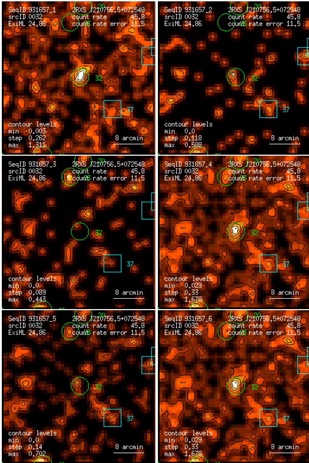
Figure 32: RASS 931657: detection 0032: band rate images, Gaussian filter: (1) PSPC channels 11 – 41, (2) 52 – 90, (3) 91 – 201, (4) 11 – 235, (5) 52 – 201, (6) 11 – 201. Broad band rates in counts/ks. Band rate contour levels in counts/ks/arcmin 2 .
