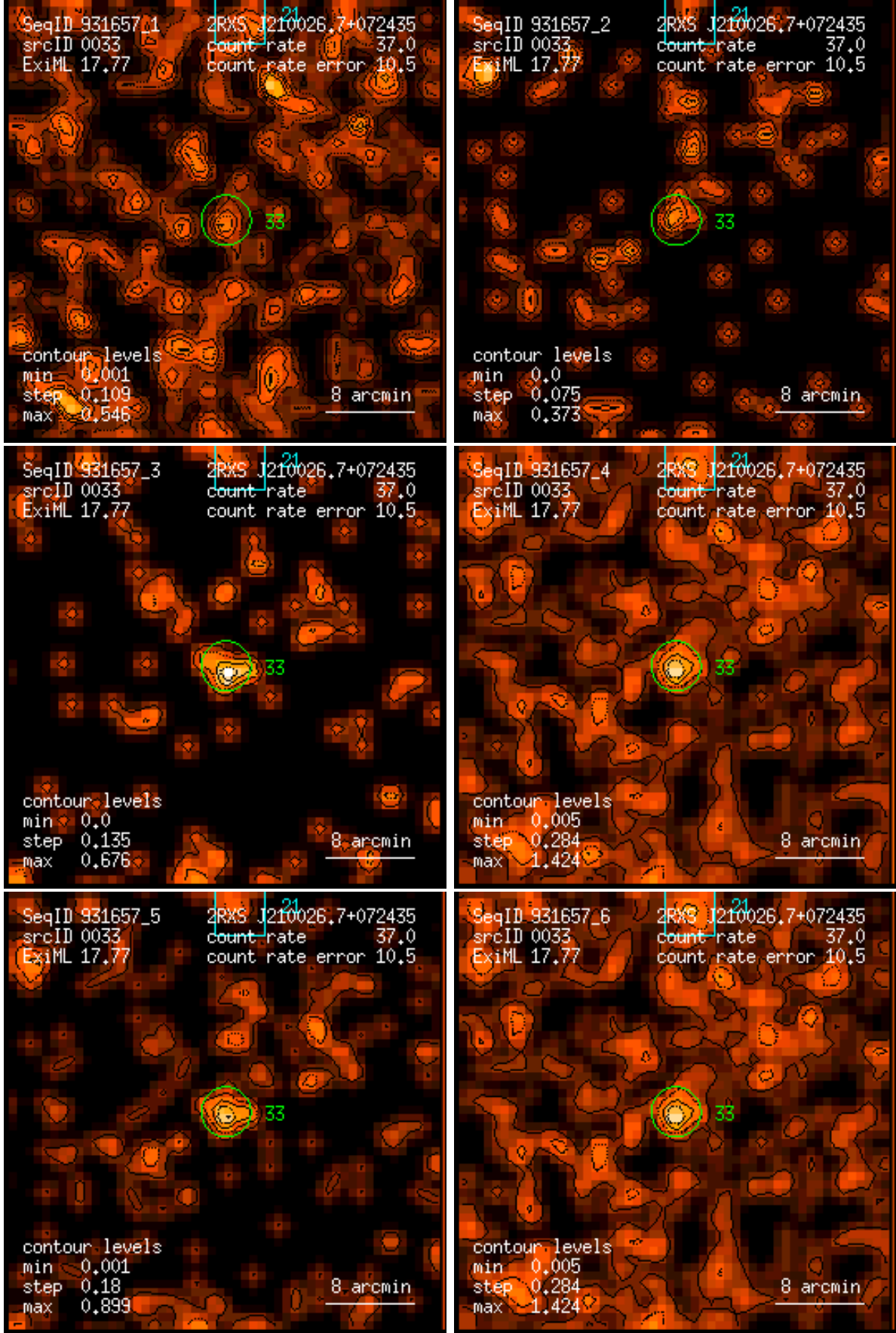
Figure 33: RASS 931657: detection 0033: band rate images, Gaussian filter: (1) PSPC channels 11 – 41, (2) 52 – 90, (3) 91 – 201, (4) 11 – 235, (5) 52 – 201, (6) 11 – 201. Broad band rates in counts/ks. Band rate contour levels in counts/ks/arcmin 2 .
