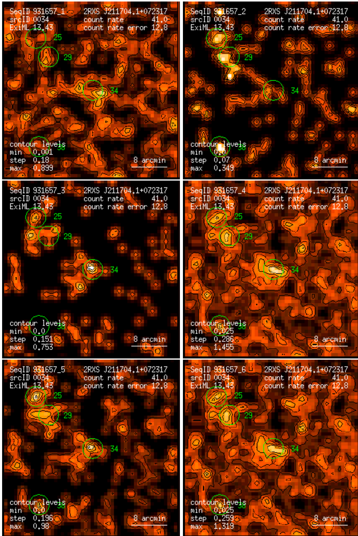
Figure 34: RASS 931657: detection 0034: band rate images, Gaussian filter: (1) PSPC channels 11 – 41, (2) 52 – 90, (3) 91 – 201, (4) 11 – 235, (5) 52 – 201, (6) 11 – 201. Broad band rates in counts/ks. Band rate contour levels in counts/ks/arcmin 2 .
