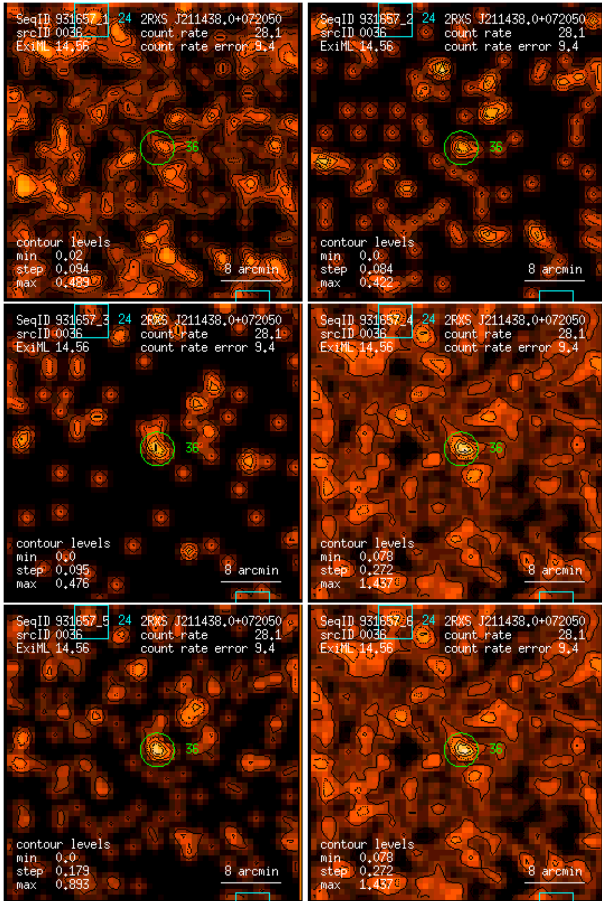
Figure 36: RASS 931657: detection 0036: band rate images, Gaussian filter: (1) PSPC channels 11 – 41, (2) 52 – 90, (3) 91 – 201, (4) 11 – 235, (5) 52 – 201, (6) 11 – 201. Broad band rates in counts/ks. Band rate contour levels in counts/ks/arcmin 2 .
