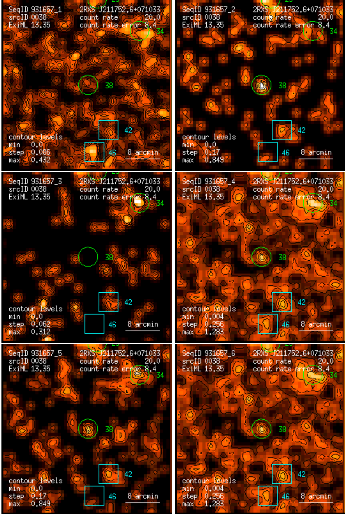
Figure 38: RASS 931657: detection 0038: band rate images, Gaussian filter: (1) PSPC channels 11 – 41, (2) 52 – 90, (3) 91 – 201, (4) 11 – 235, (5) 52 – 201, (6) 11 – 201. Broad band rates in counts/ks. Band rate contour levels in counts/ks/arcmin 2 .
