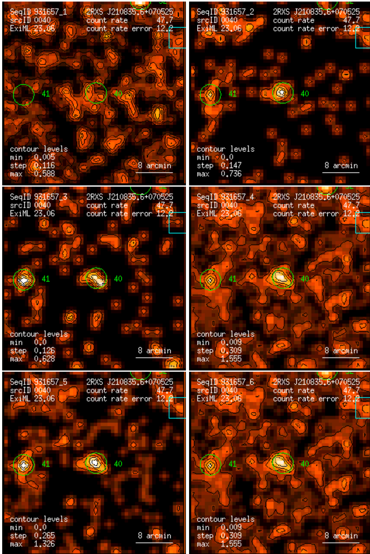
Figure 40: RASS 931657: detection 0040: band rate images, Gaussian filter: (1) PSPC channels 11 – 41, (2) 52 – 90, (3) 91 – 201, (4) 11 – 235, (5) 52 – 201, (6) 11 – 201. Broad band rates in counts/ks. Band rate contour levels in counts/ks/arcmin 2 .
