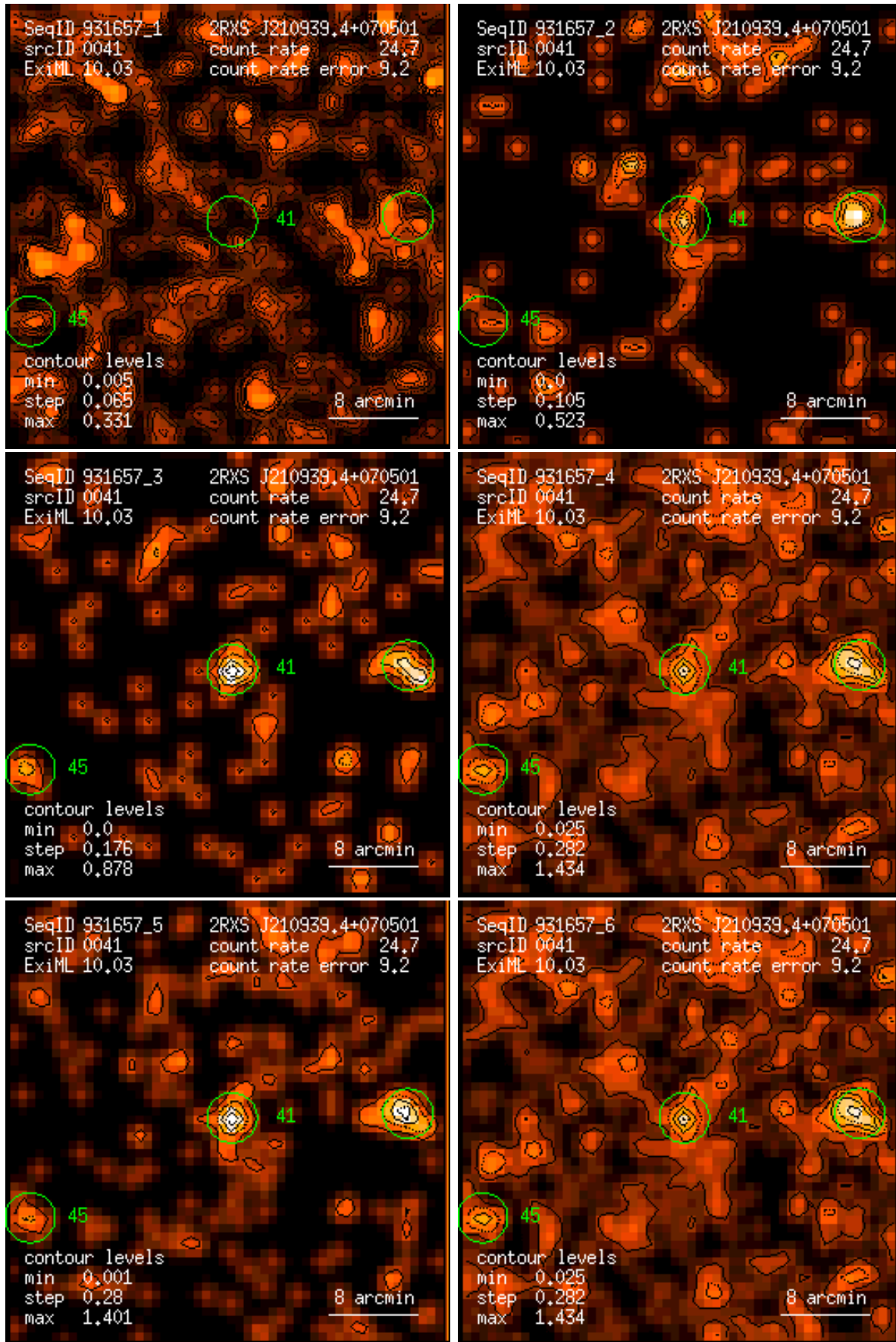
Figure 41: RASS 931657: detection 0041: band rate images, Gaussian filter: (1) PSPC channels 11 – 41, (2) 52 – 90, (3) 91 – 201, (4) 11 – 235, (5) 52 – 201, (6) 11 – 201. Broad band rates in counts/ks. Band rate contour levels in counts/ks/arcmin 2 .
