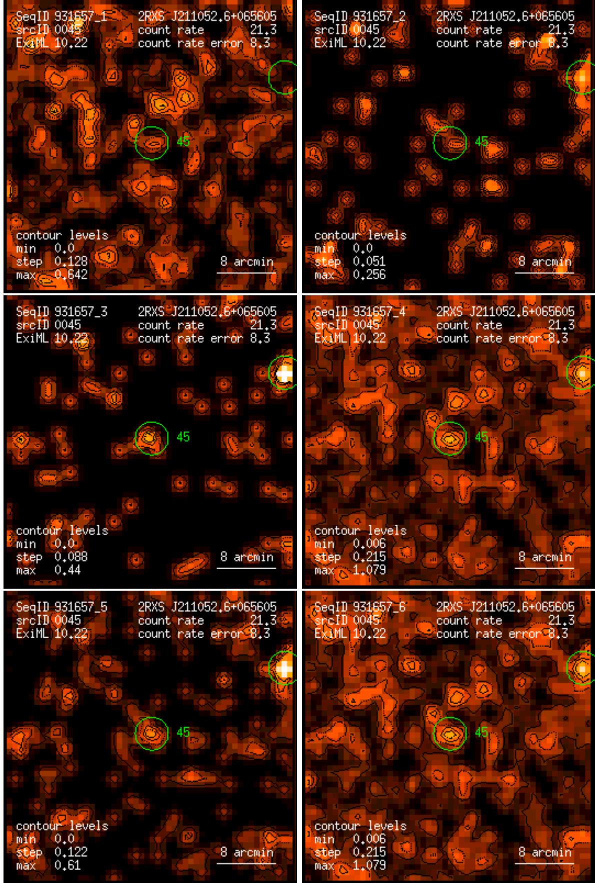
Figure 45: RASS 931657: detection 0045: band rate images, Gaussian filter: (1) PSPC channels 11 – 41, (2) 52 – 90, (3) 91 – 201, (4) 11 – 235, (5) 52 – 201, (6) 11 – 201. Broad band rates in counts/ks. Band rate contour levels in counts/ks/arcmin 2 .
