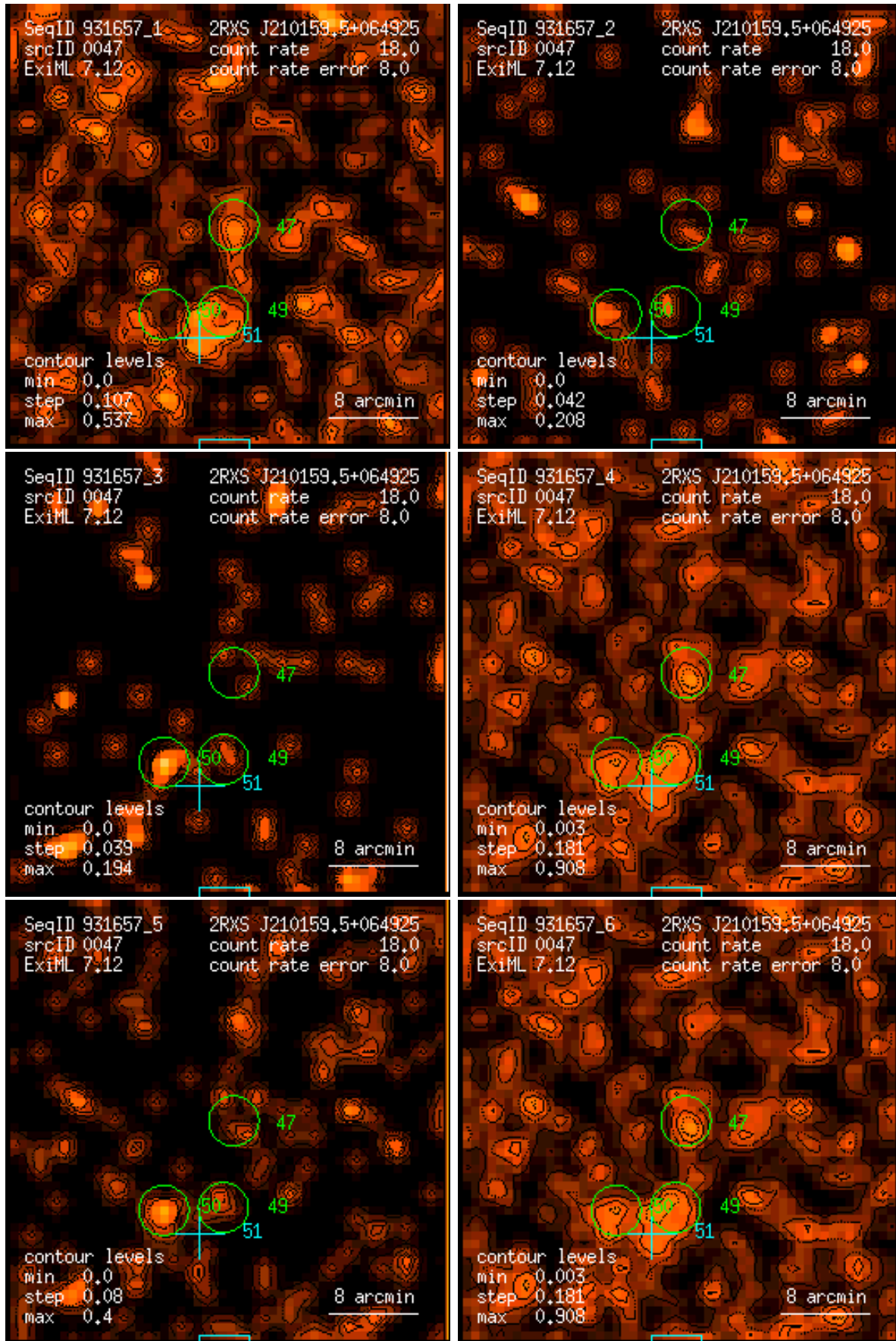
Figure 47: RASS 931657: detection 0047: band rate images, Gaussian filter: (1) PSPC channels 11 – 41, (2) 52 – 90, (3) 91 – 201, (4) 11 – 235, (5) 52 – 201, (6) 11 – 201. Broad band rates in counts/ks. Band rate contour levels in counts/ks/arcmin 2 .
