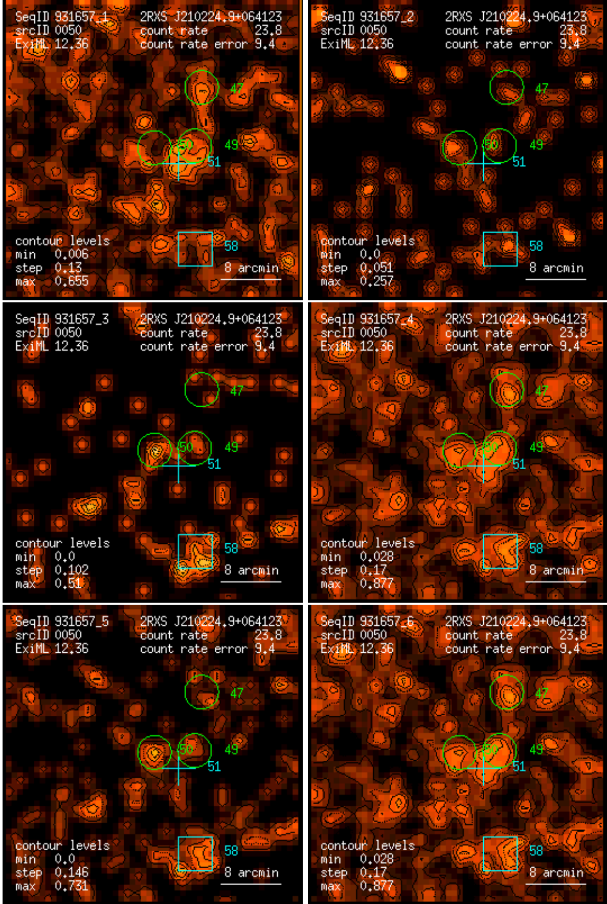
Figure 50: RASS 931657: detection 0050: band rate images, Gaussian filter: (1) PSPC channels 11 – 41, (2) 52 – 90, (3) 91 – 201, (4) 11 – 235, (5) 52 – 201, (6) 11 – 201. Broad band rates in counts/ks. Band rate contour levels in counts/ks/arcmin 2 .
