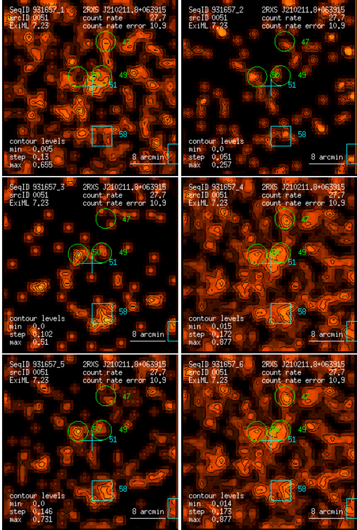
Figure 51: RASS 931657: detection 0051: band rate images, Gaussian filter: (1) PSPC channels 11 – 41, (2) 52 – 90, (3) 91 – 201, (4) 11 – 235, (5) 52 – 201, (6) 11 – 201. Broad band rates in counts/ks. Band rate contour levels in counts/ks/arcmin 2 .
