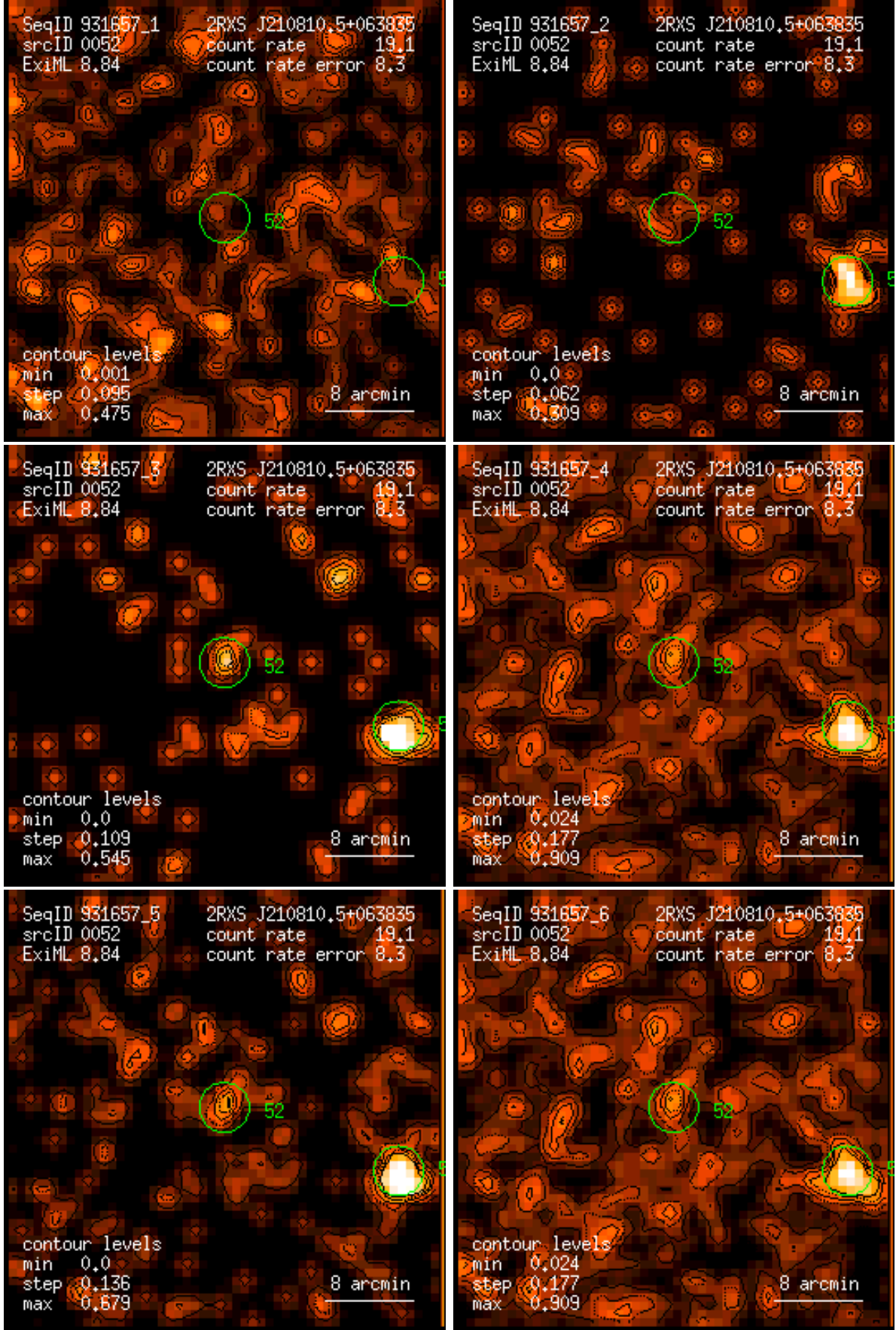
Figure 52: RASS 931657: detection 0052: band rate images, Gaussian filter: (1) PSPC channels 11 – 41, (2) 52 – 90, (3) 91 – 201, (4) 11 – 235, (5) 52 – 201, (6) 11 – 201. Broad band rates in counts/ks. Band rate contour levels in counts/ks/arcmin 2 .
