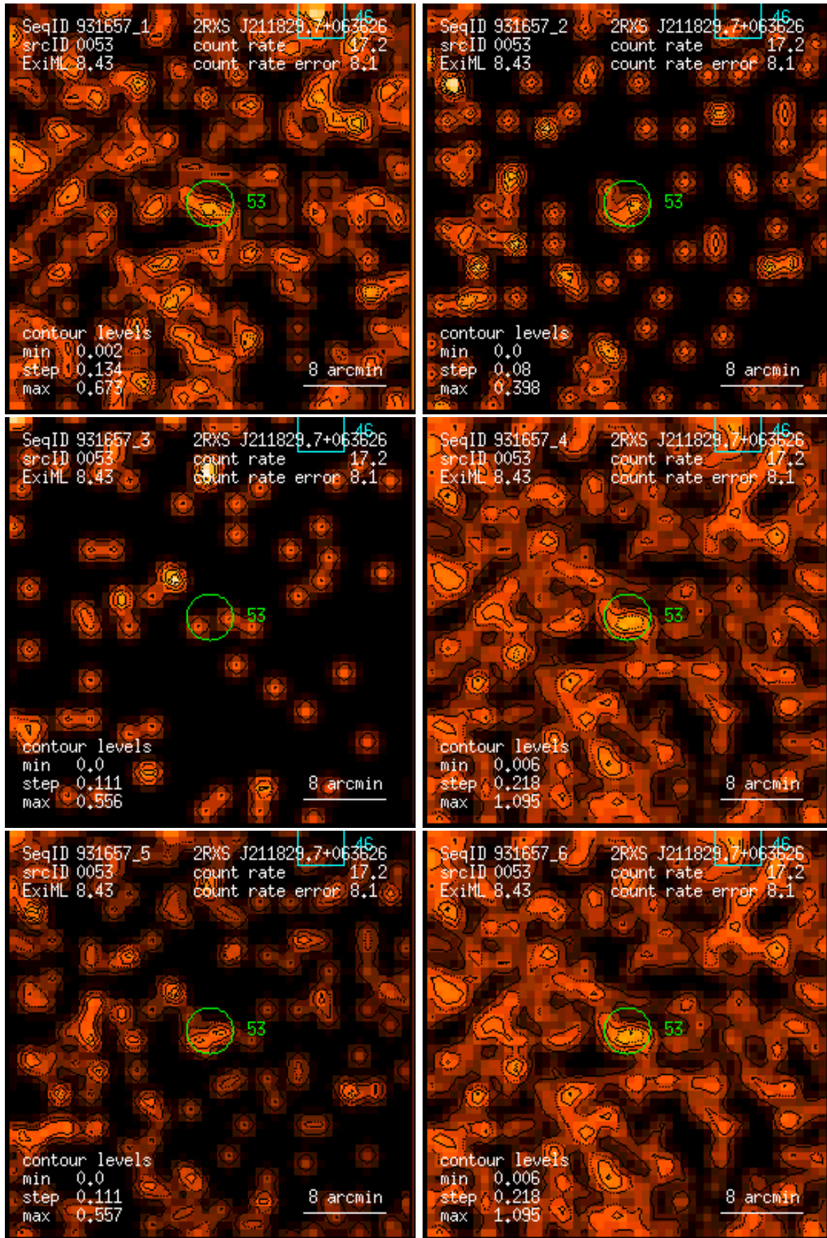
Figure 53: RASS 931657: detection 0053: band rate images, Gaussian filter: (1) PSPC channels 11 – 41, (2) 52 – 90, (3) 91 – 201, (4) 11 – 235, (5) 52 – 201, (6) 11 – 201. Broad band rates in counts/ks. Band rate contour levels in counts/ks/arcmin 2 .
