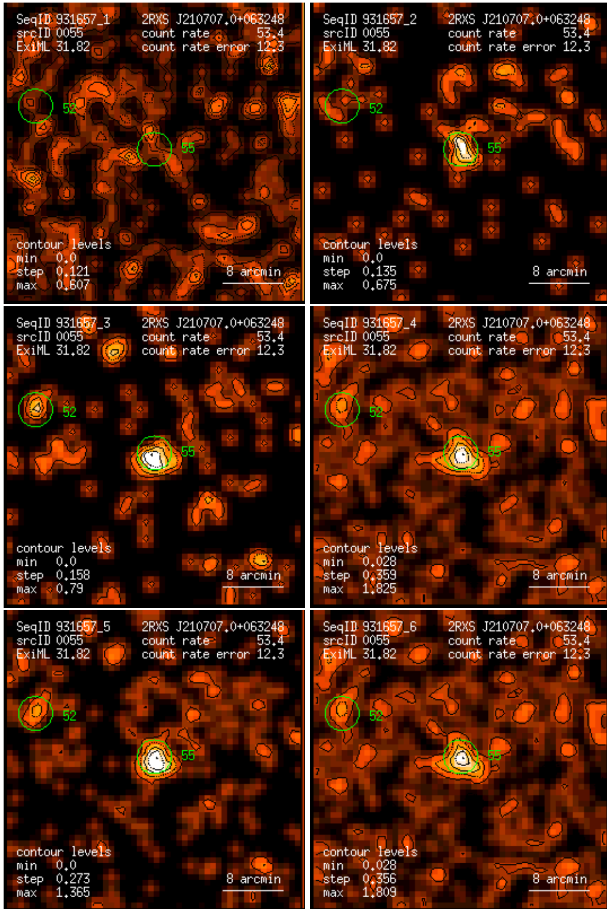
Figure 55: RASS 931657: detection 0055: band rate images, Gaussian filter: (1) PSPC channels 11 – 41, (2) 52 – 90, (3) 91 – 201, (4) 11 – 235, (5) 52 – 201, (6) 11 – 201. Broad band rates in counts/ks. Band rate contour levels in counts/ks/arcmin 2 .
